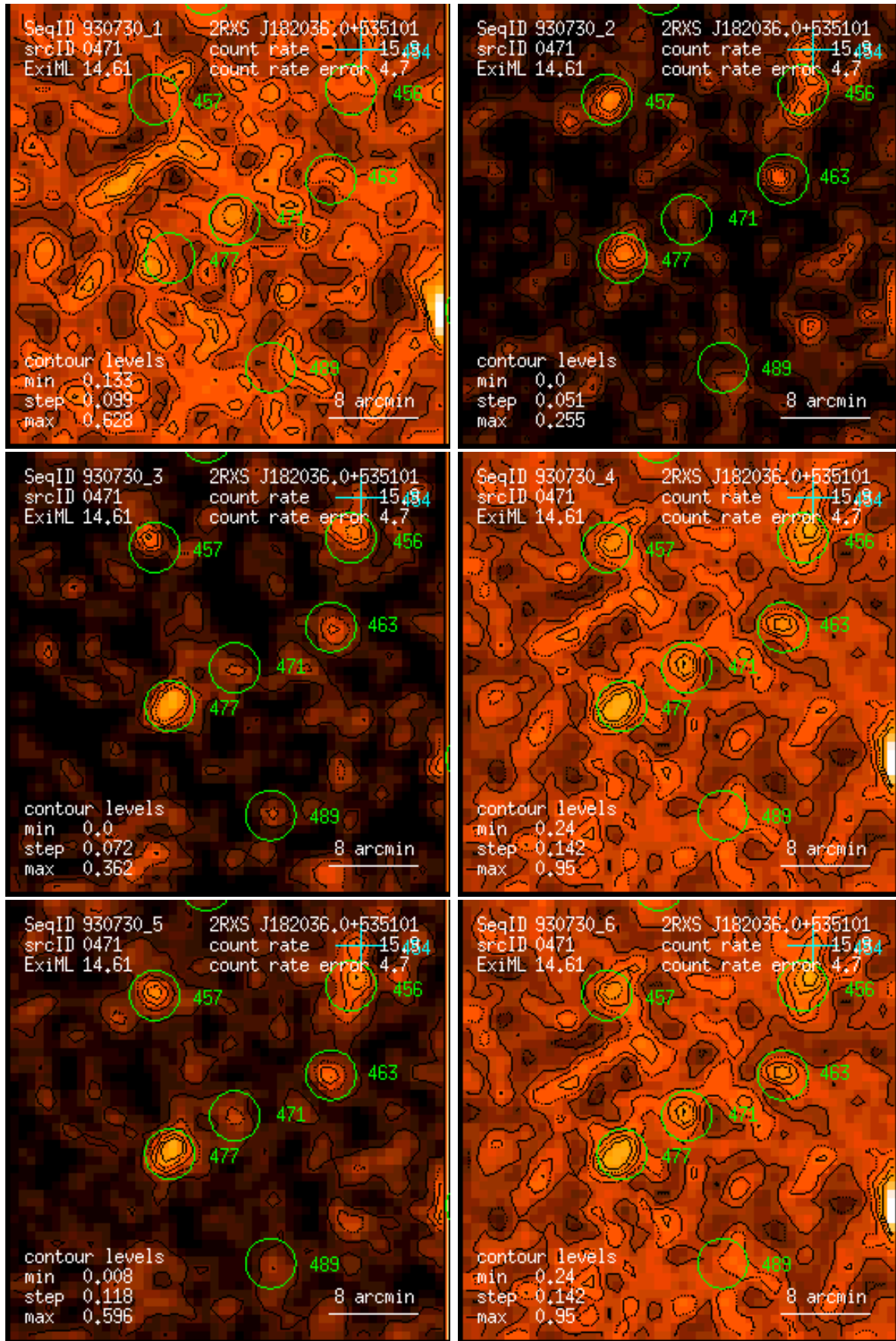
Figure 471: RASS 930730: detection 0471: band rate images, Gaussian filter: (1) PSPC channels 11 – 41, (2) 52 – 90, (3) 91 – 201, (4) 11 – 235, (5) 52 – 201, (6) 11 – 201. Broad band rates in counts/ks. Band rate contour levels in counts/ks/arcmin 2 .
