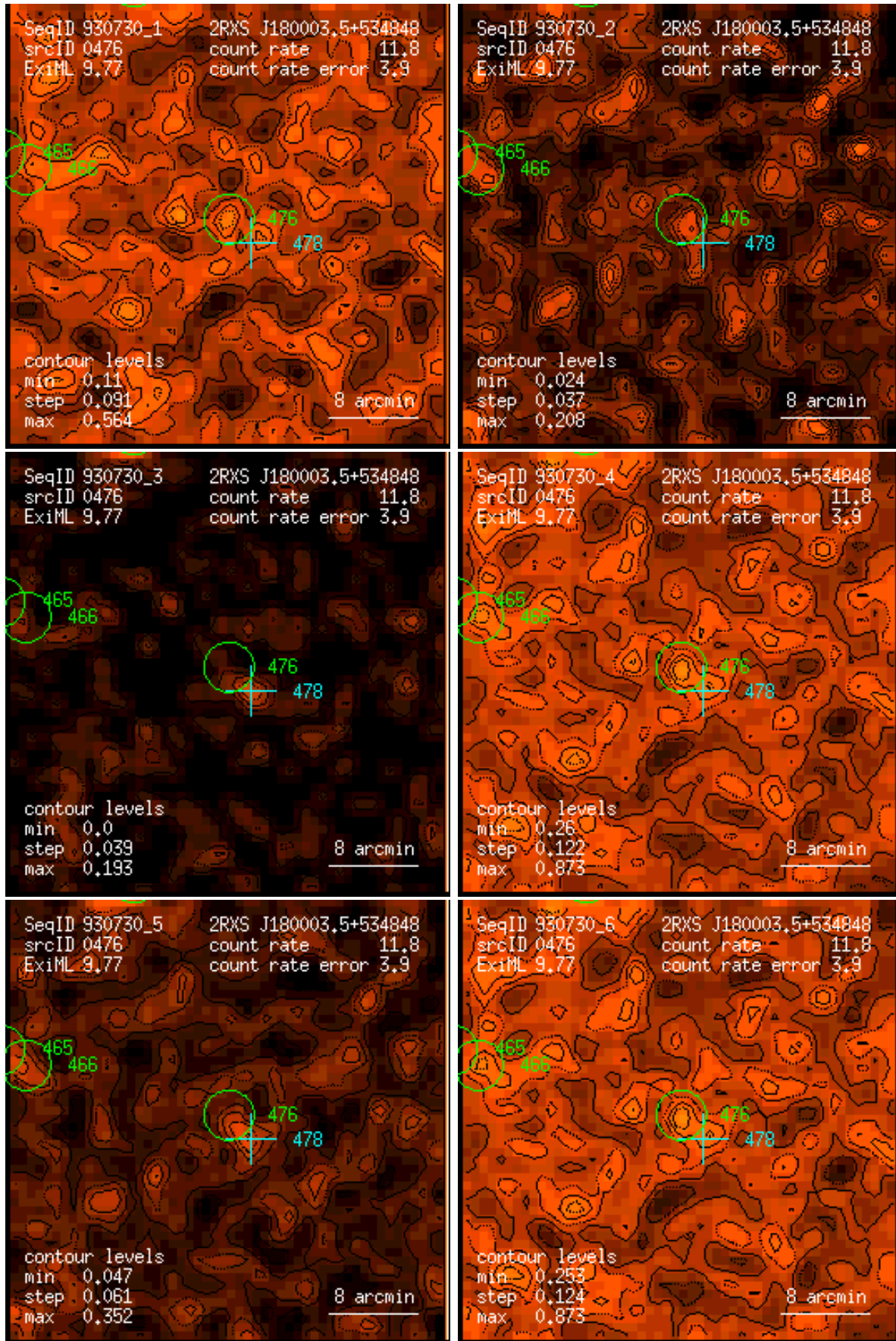
Figure 476: RASS 930730: detection 0476: band rate images, Gaussian filter: (1) PSPC channels 11 – 41, (2) 52 – 90, (3) 91 – 201, (4) 11 – 235, (5) 52 – 201, (6) 11 – 201. Broad band rates in counts/ks. Band rate contour levels in counts/ks/arcmin 2 .
