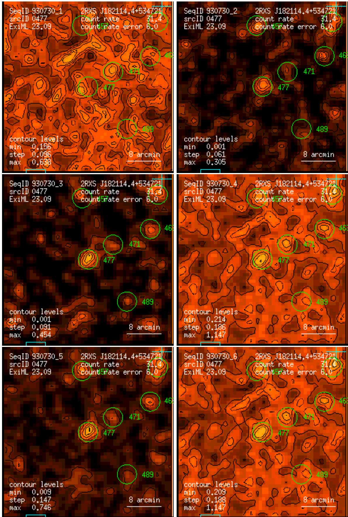
Figure 477: RASS 930730: detection 0477: band rate images, Gaussian filter: (1) PSPC channels 11 – 41, (2) 52 – 90, (3) 91 – 201, (4) 11 – 235, (5) 52 – 201, (6) 11 – 201. Broad band rates in counts/ks. Band rate contour levels in counts/ks/arcmin 2 .
