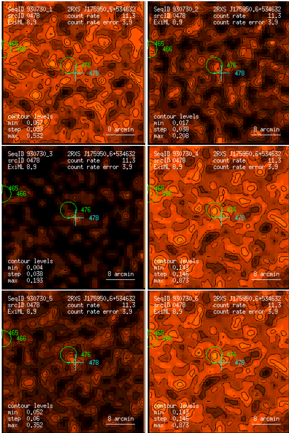
Figure 478: RASS 930730: detection 0478: band rate images, Gaussian filter: (1) PSPC channels 11 – 41, (2) 52 – 90, (3) 91 – 201, (4) 11 – 235, (5) 52 – 201, (6) 11 – 201. Broad band rates in counts/ks. Band rate contour levels in counts/ks/arcmin 2 .
