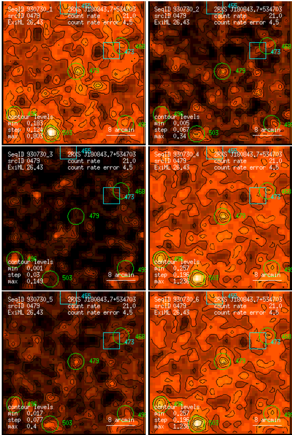
Figure 479: RASS 930730: detection 0479: band rate images, Gaussian filter: (1) PSPC channels 11 – 41, (2) 52 – 90, (3) 91 – 201, (4) 11 – 235, (5) 52 – 201, (6) 11 – 201. Broad band rates in counts/ks. Band rate contour levels in counts/ks/arcmin 2 .
