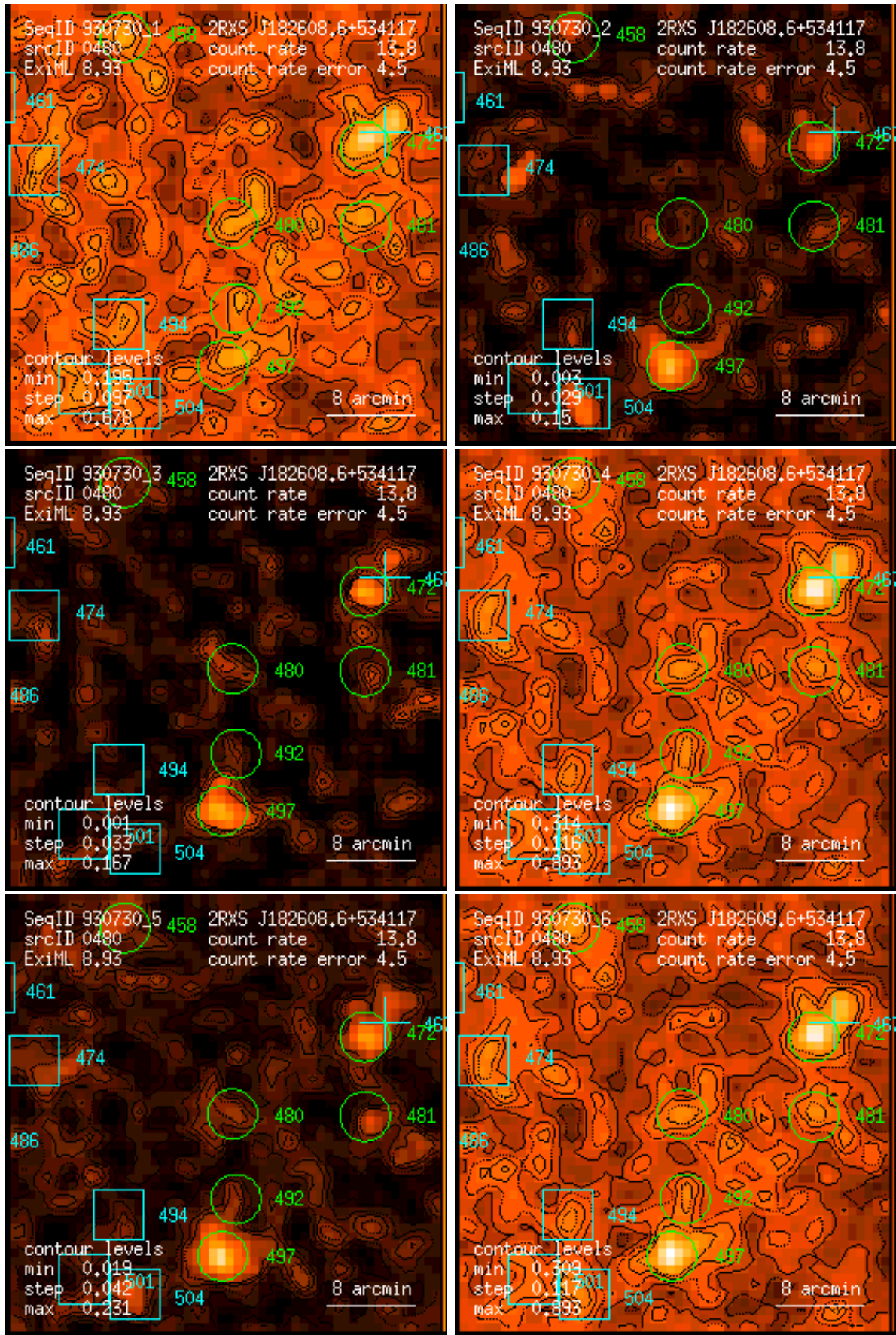
Figure 480: RASS 930730: detection 0480: band rate images, Gaussian filter: (1) PSPC channels 11 – 41, (2) 52 – 90, (3) 91 – 201, (4) 11 – 235, (5) 52 – 201, (6) 11 – 201. Broad band rates in counts/ks. Band rate contour levels in counts/ks/arcmin 2 .
