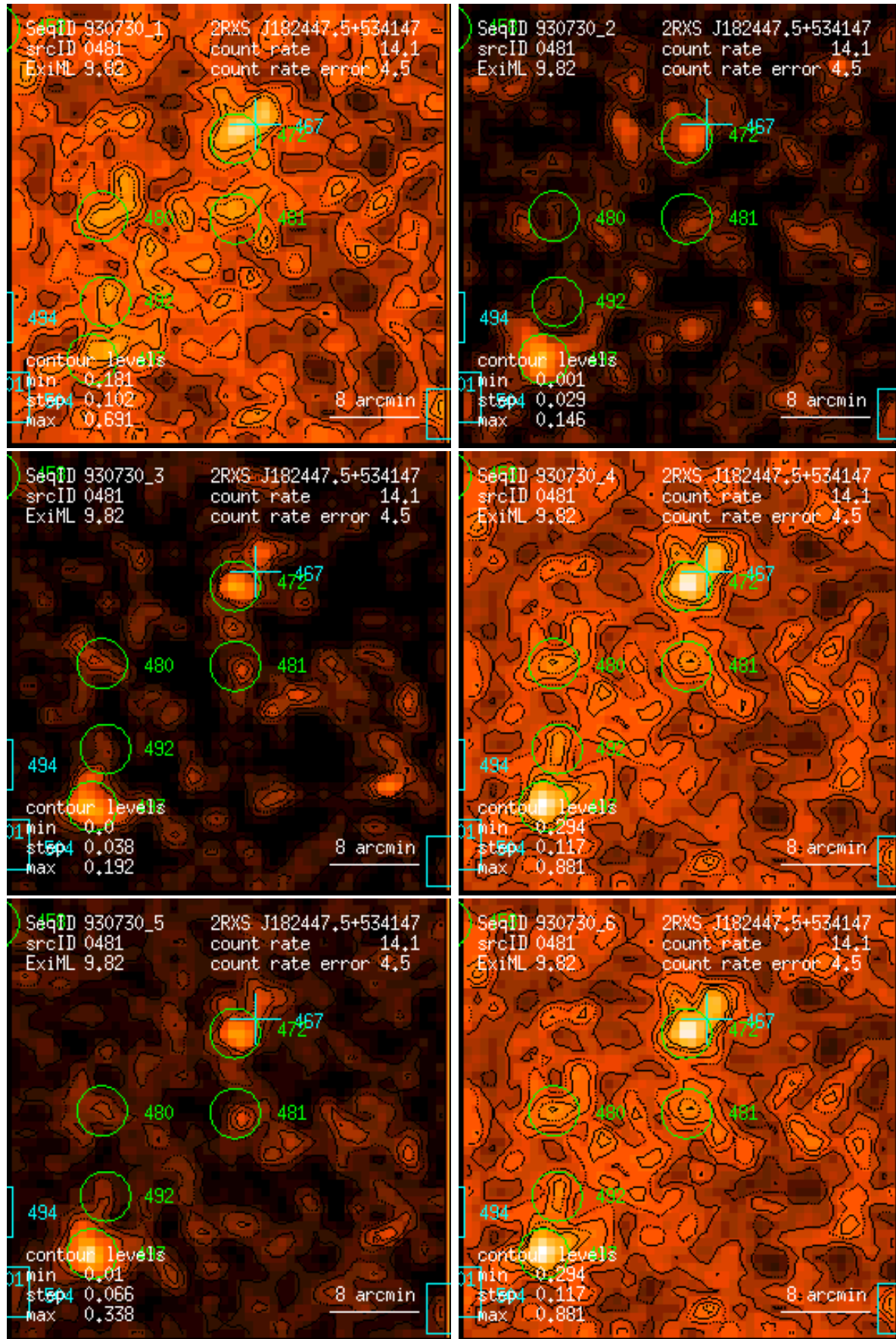
Figure 481: RASS 930730: detection 0481: band rate images, Gaussian filter: (1) PSPC channels 11 – 41, (2) 52 – 90, (3) 91 – 201, (4) 11 – 235, (5) 52 – 201, (6) 11 – 201. Broad band rates in counts/ks. Band rate contour levels in counts/ks/arcmin 2 .
