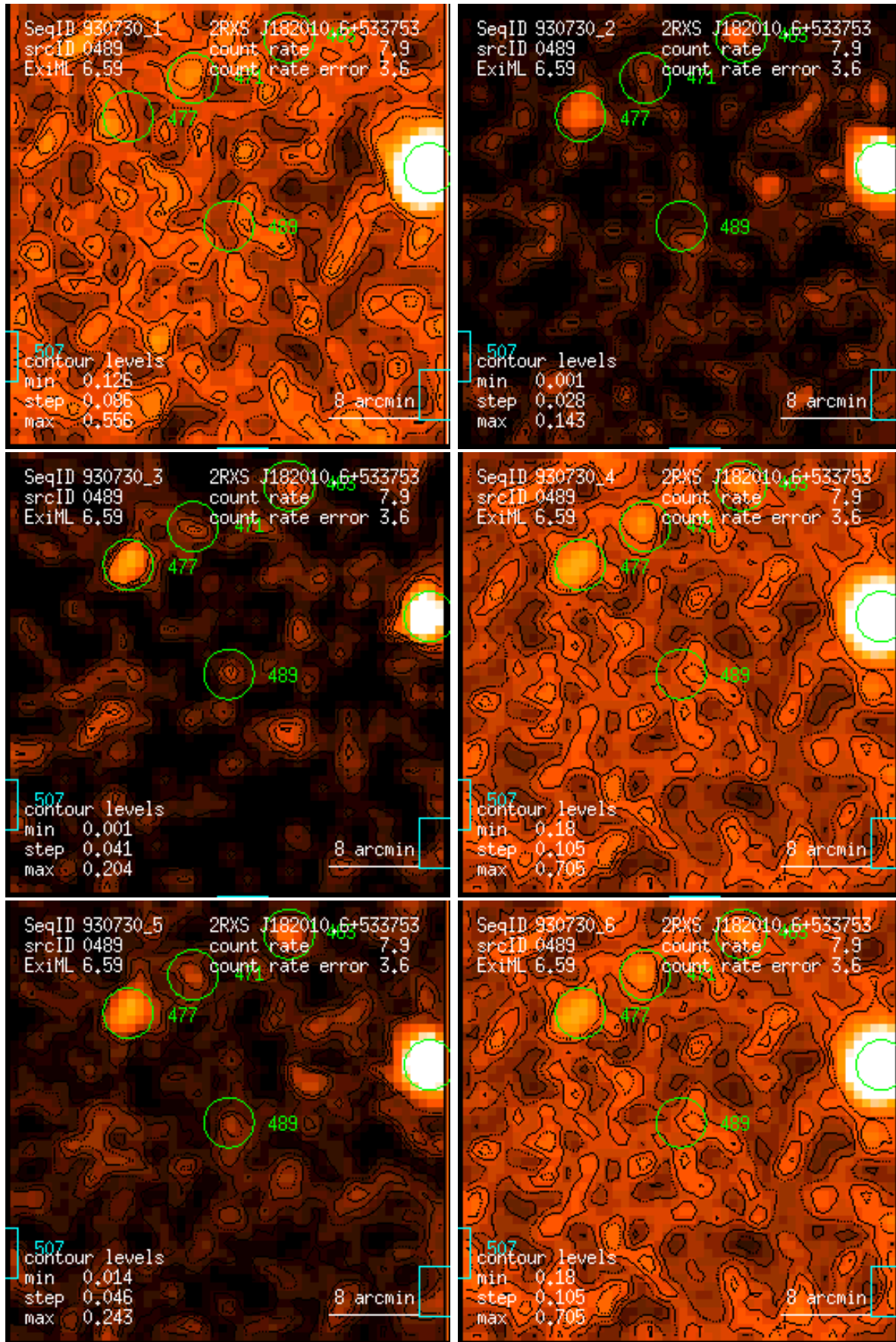
Figure 489: RASS 930730: detection 0489: band rate images, Gaussian filter: (1) PSPC channels 11 – 41, (2) 52 – 90, (3) 91 – 201, (4) 11 – 235, (5) 52 – 201, (6) 11 – 201. Broad band rates in counts/ks. Band rate contour levels in counts/ks/arcmin 2 .
