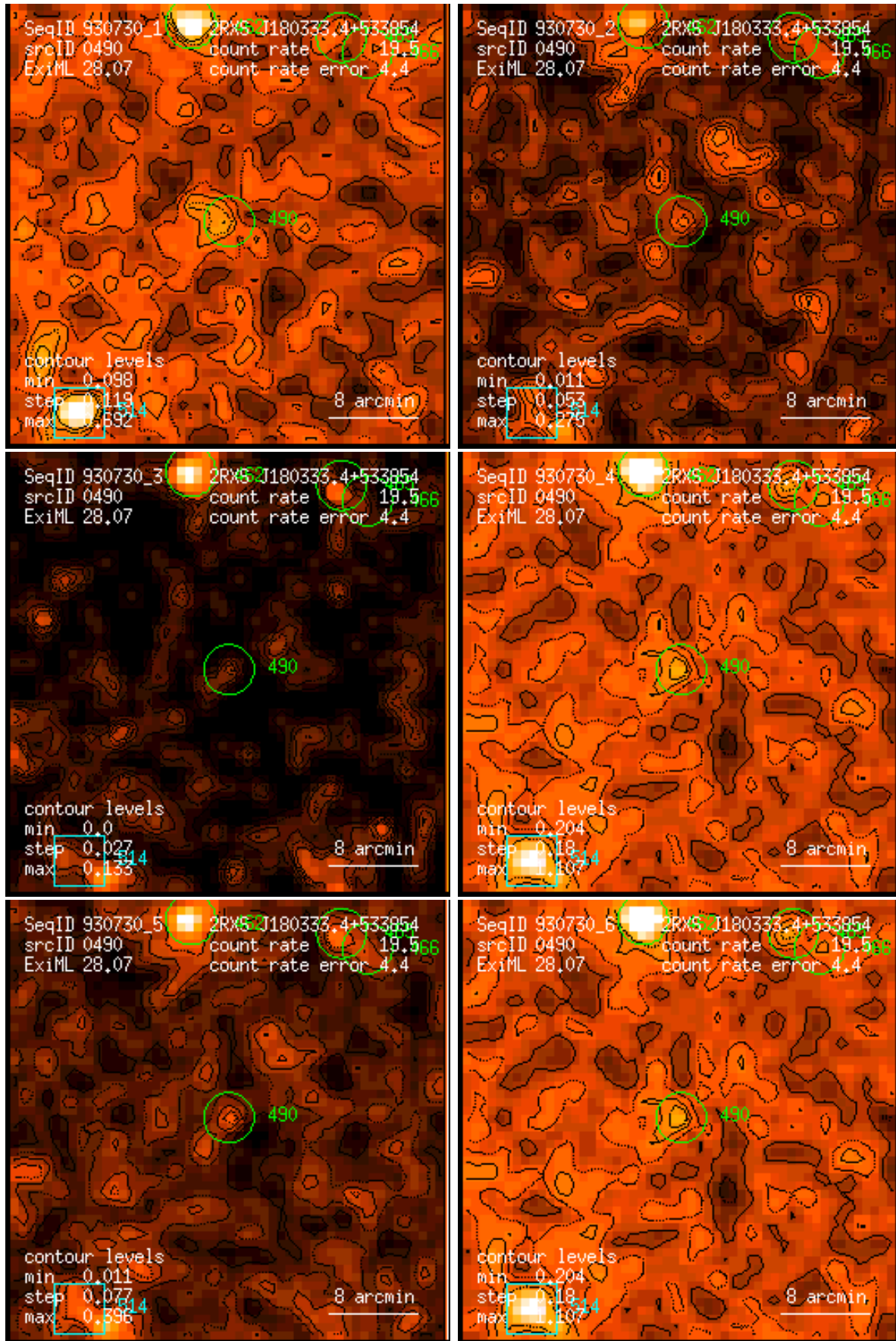
Figure 490: RASS 930730: detection 0490: band rate images, Gaussian filter: (1) PSPC channels 11 – 41, (2) 52 – 90, (3) 91 – 201, (4) 11 – 235, (5) 52 – 201, (6) 11 – 201. Broad band rates in counts/ks. Band rate contour levels in counts/ks/arcmin 2 .
