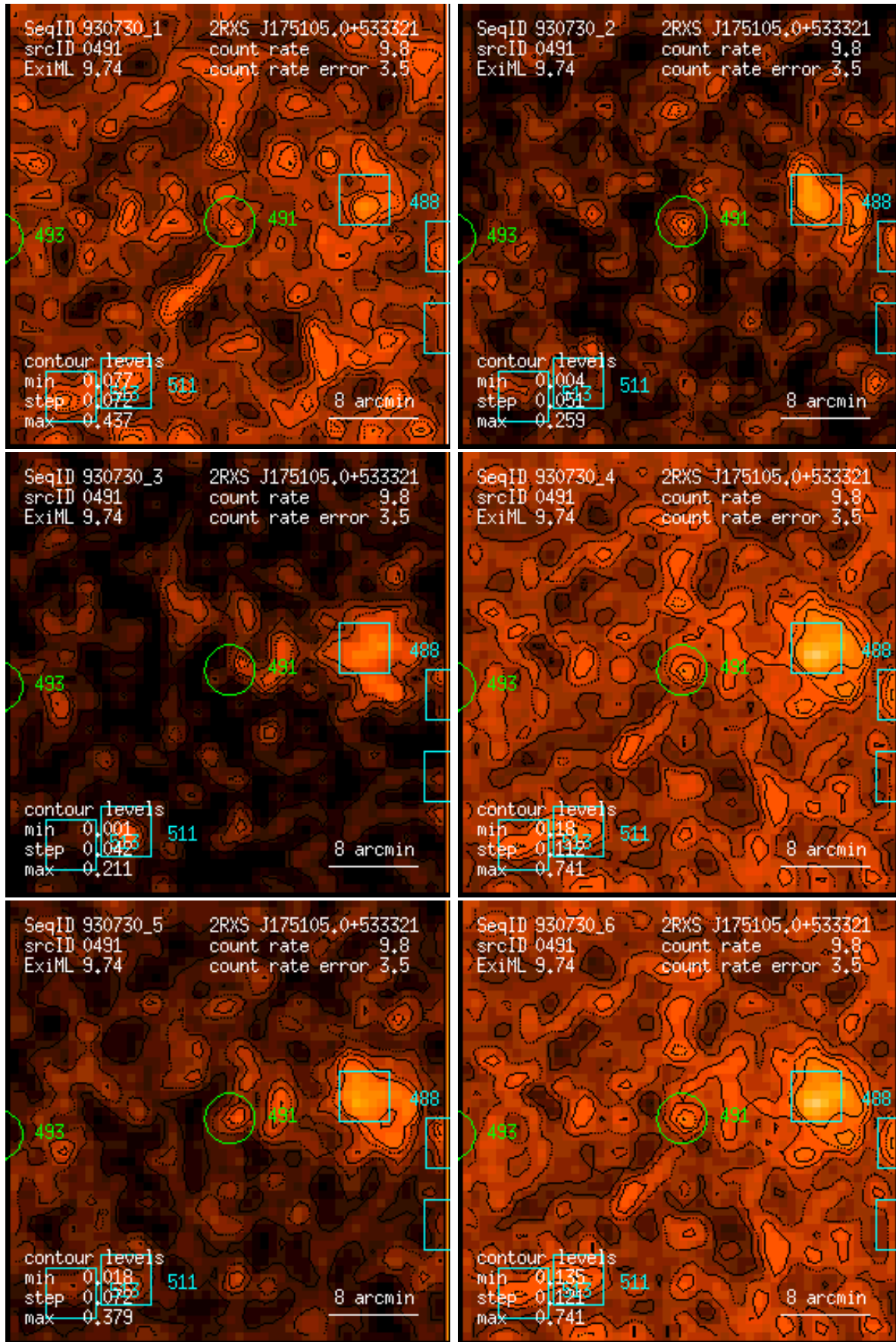
Figure 491: RASS 930730: detection 0491: band rate images, Gaussian filter: (1) PSPC channels 11 – 41, (2) 52 – 90, (3) 91 – 201, (4) 11 – 235, (5) 52 – 201, (6) 11 – 201. Broad band rates in counts/ks. Band rate contour levels in counts/ks/arcmin 2 .
