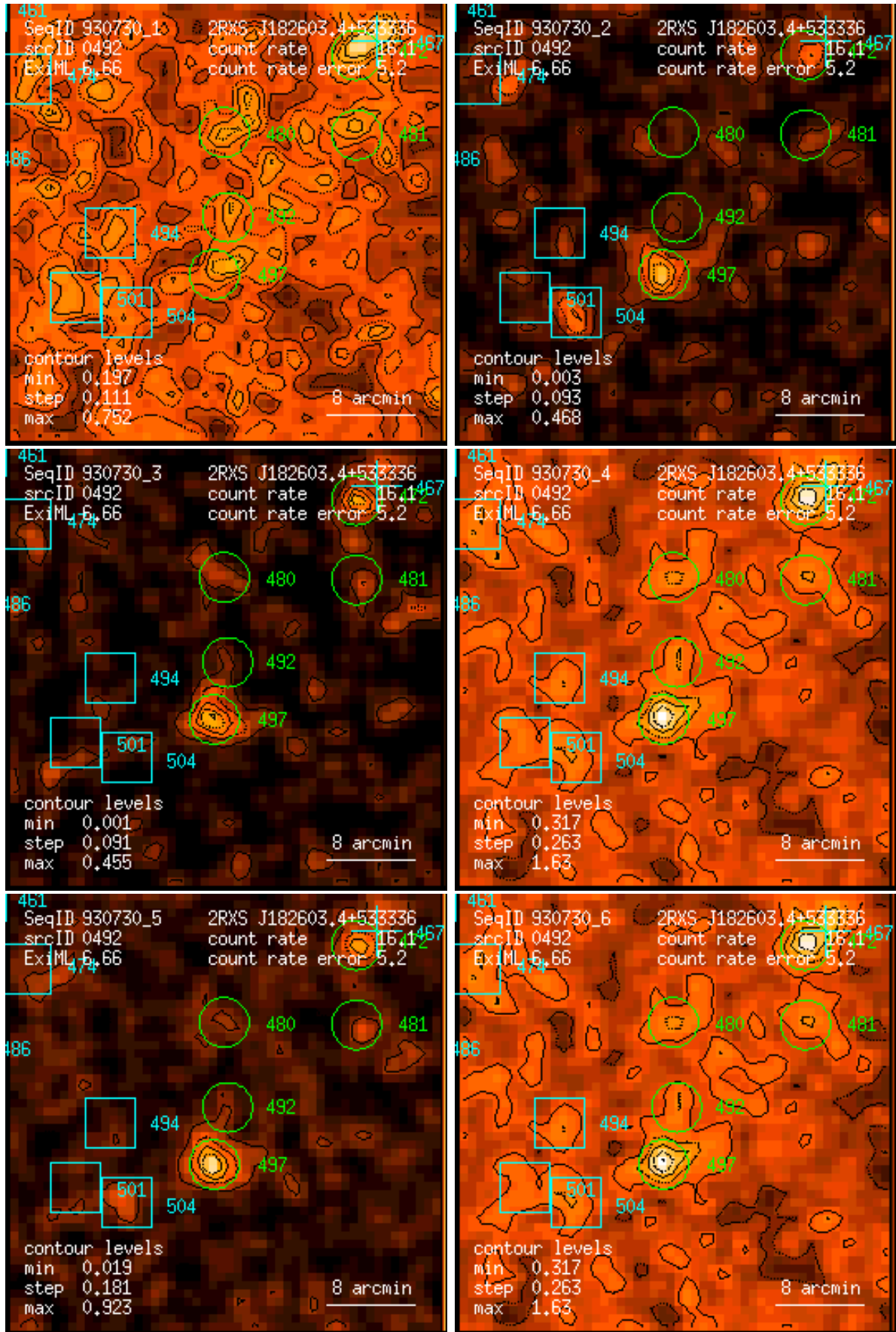
Figure 492: RASS 930730: detection 0492: band rate images, Gaussian filter: (1) PSPC channels 11 – 41, (2) 52 – 90, (3) 91 – 201, (4) 11 – 235, (5) 52 – 201, (6) 11 – 201. Broad band rates in counts/ks. Band rate contour levels in counts/ks/arcmin 2 .
