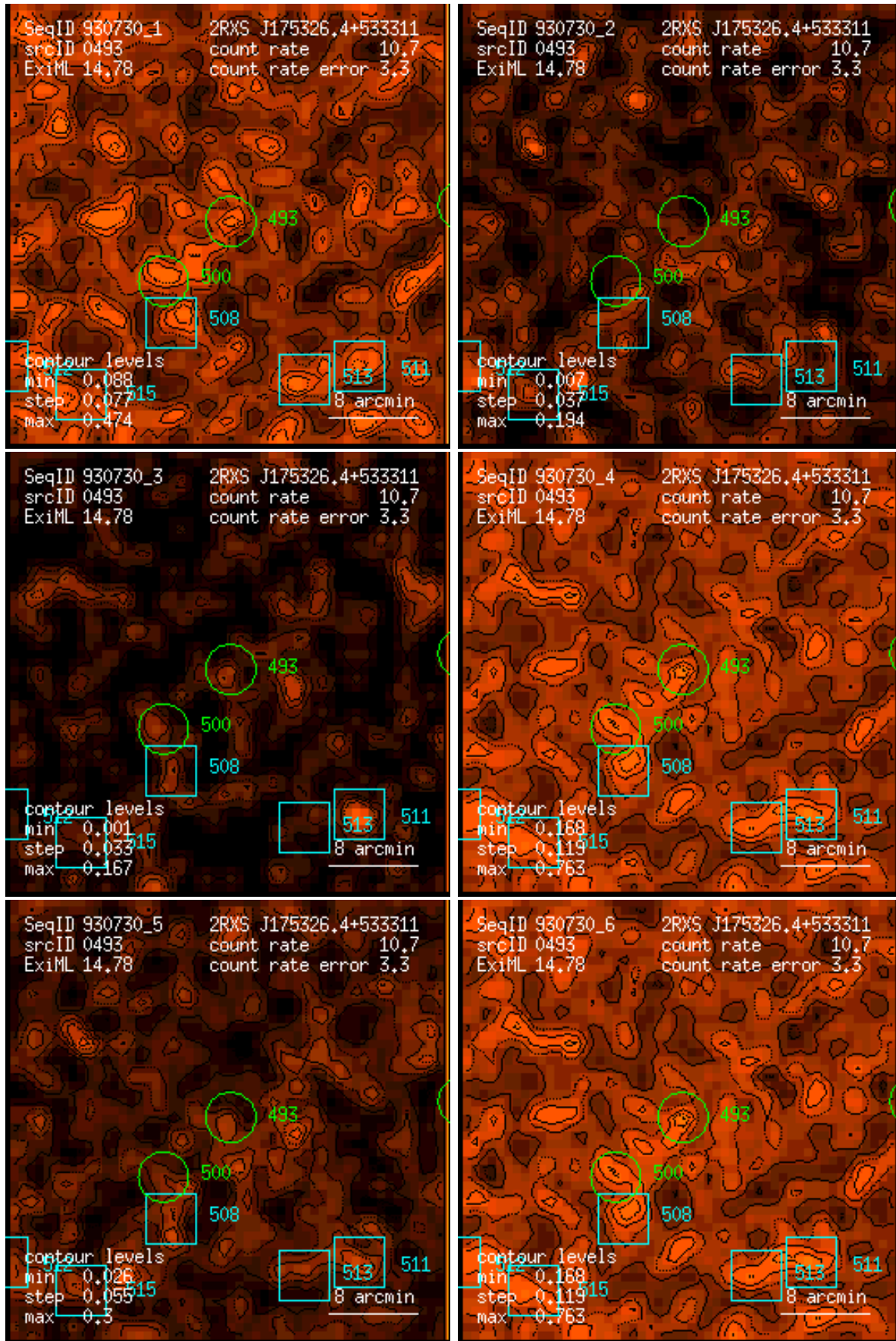
Figure 493: RASS 930730: detection 0493: band rate images, Gaussian filter: (1) PSPC channels 11 – 41, (2) 52 – 90, (3) 91 – 201, (4) 11 – 235, (5) 52 – 201, (6) 11 – 201. Broad band rates in counts/ks. Band rate contour levels in counts/ks/arcmin 2 .
