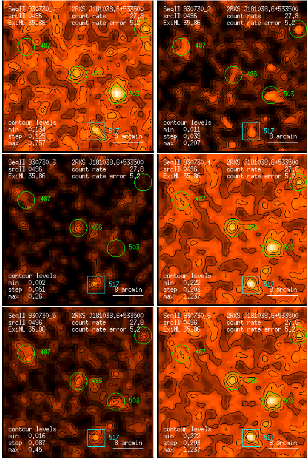
Figure 496: RASS 930730: detection 0496: band rate images, Gaussian filter: (1) PSPC channels 11 – 41, (2) 52 – 90, (3) 91 – 201, (4) 11 – 235, (5) 52 – 201, (6) 11 – 201. Broad band rates in counts/ks. Band rate contour levels in counts/ks/arcmin 2 .
