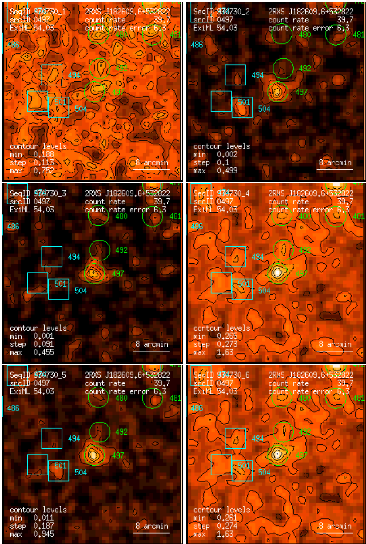
Figure 497: RASS 930730: detection 0497: band rate images, Gaussian filter: (1) PSPC channels 11 – 41, (2) 52 – 90, (3) 91 – 201, (4) 11 – 235, (5) 52 – 201, (6) 11 – 201. Broad band rates in counts/ks. Band rate contour levels in counts/ks/arcmin 2 .
