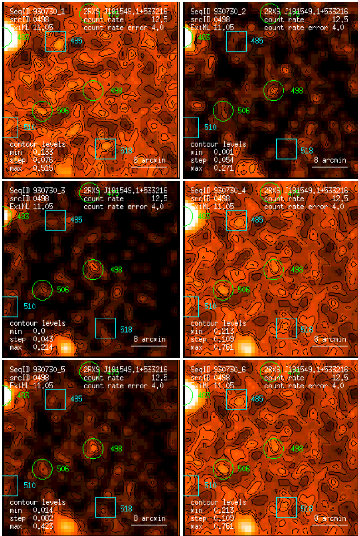
Figure 498: RASS 930730: detection 0498: band rate images, Gaussian filter: (1) PSPC channels 11 – 41, (2) 52 – 90, (3) 91 – 201, (4) 11 – 235, (5) 52 – 201, (6) 11 – 201. Broad band rates in counts/ks. Band rate contour levels in counts/ks/arcmin 2 .
