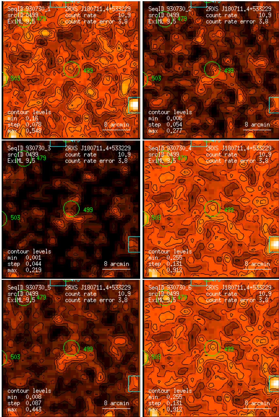
Figure 499: RASS 930730: detection 0499: band rate images, Gaussian filter: (1) PSPC channels 11 – 41, (2) 52 – 90, (3) 91 – 201, (4) 11 – 235, (5) 52 – 201, (6) 11 – 201. Broad band rates in counts/ks. Band rate contour levels in counts/ks/arcmin 2 .
