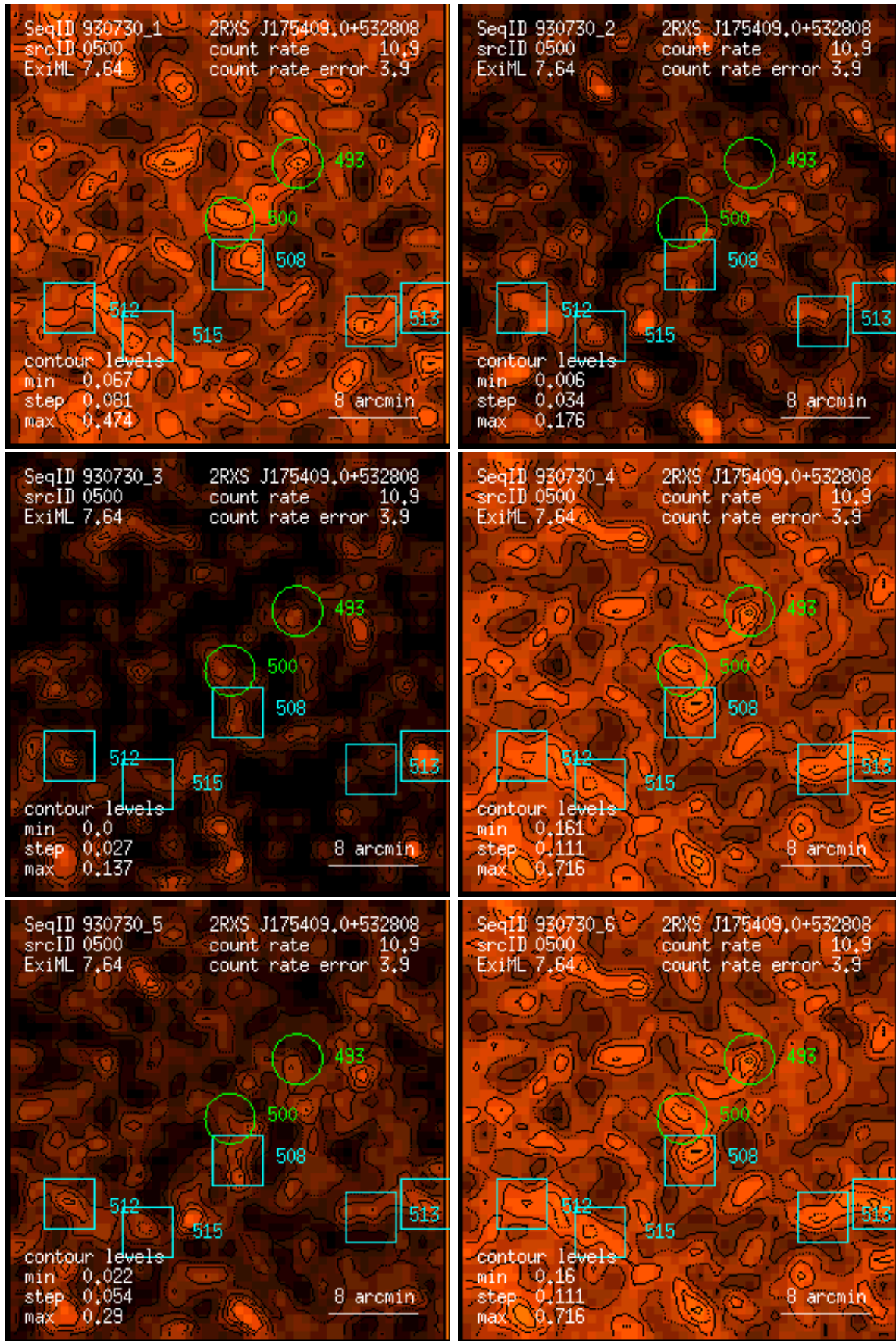
Figure 500: RASS 930730: detection 0500: band rate images, Gaussian filter: (1) PSPC channels 11 – 41, (2) 52 – 90, (3) 91 – 201, (4) 11 – 235, (5) 52 – 201, (6) 11 – 201. Broad band rates in counts/ks. Band rate contour levels in counts/ks/arcmin 2 .
