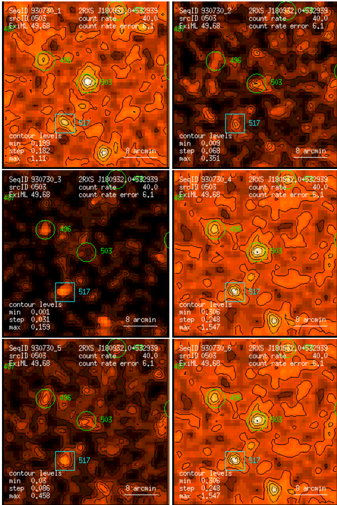
Figure 503: RASS 930730: detection 0503: band rate images, Gaussian filter: (1) PSPC channels 11 – 41, (2) 52 – 90, (3) 91 – 201, (4) 11 – 235, (5) 52 – 201, (6) 11 – 201. Broad band rates in counts/ks. Band rate contour levels in counts/ks/arcmin 2 .
