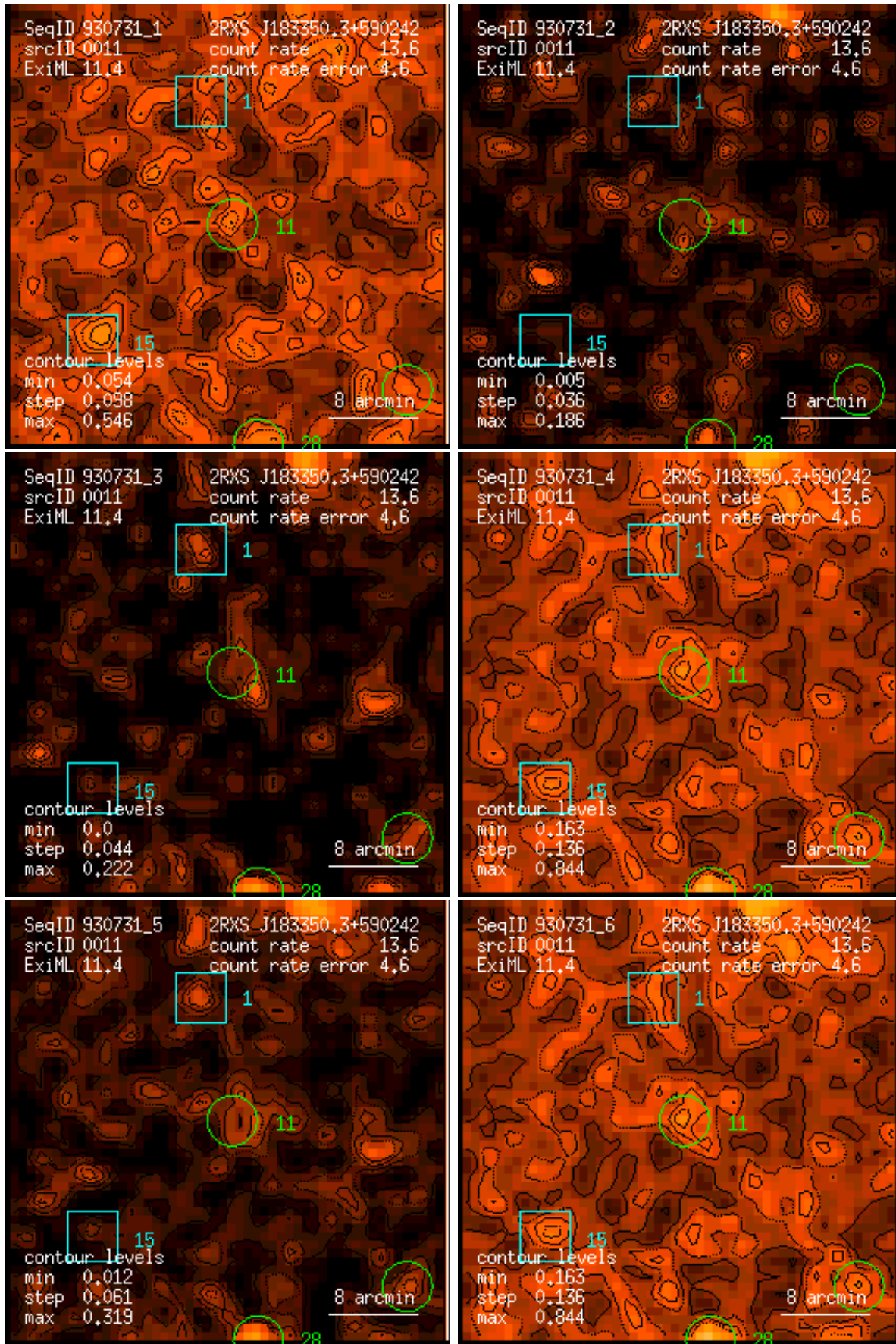
Figure 11: RASS 930731: detection 0011: band rate images, Gaussian filter: (1) PSPC channels 11 – 41, (2) 52 – 90, (3) 91 – 201, (4) 11 – 235, (5) 52 – 201, (6) 11 – 201. Broad band rates in counts/ks. Band rate contour levels in counts/ks/arcmin 2 .
