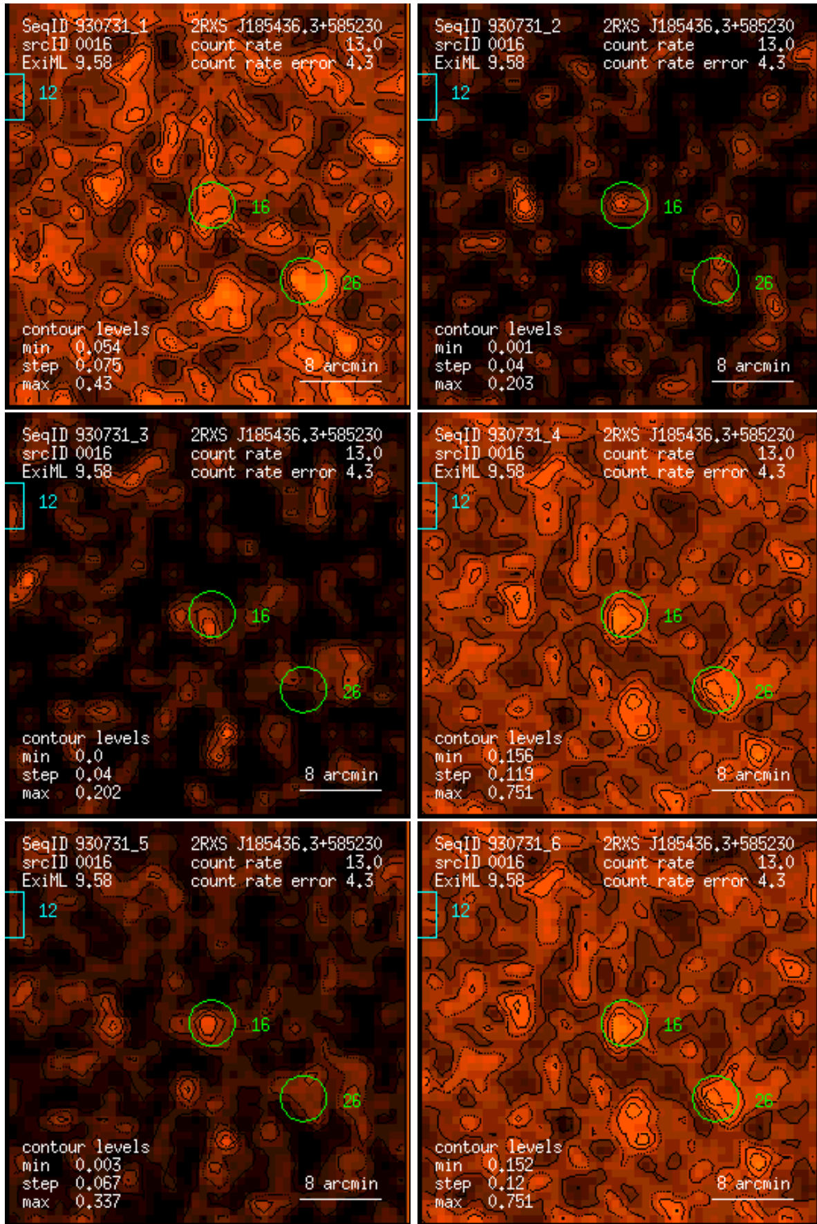
Figure 16: RASS 930731: detection 0016: band rate images, Gaussian filter: (1) PSPC channels 11 – 41, (2) 52 – 90, (3) 91 – 201, (4) 11 – 235, (5) 52 – 201, (6) 11 – 201. Broad band rates in counts/ks. Band rate contour levels in counts/ks/arcmin 2 .
