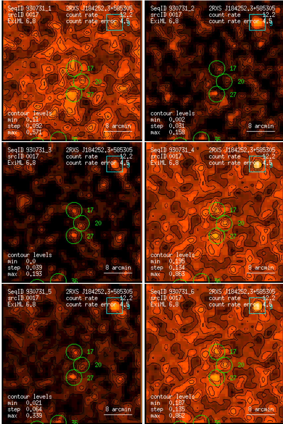
Figure 17: RASS 930731: detection 0017: band rate images, Gaussian filter: (1) PSPC channels 11 – 41, (2) 52 – 90, (3) 91 – 201, (4) 11 – 235, (5) 52 – 201, (6) 11 – 201. Broad band rates in counts/ks. Band rate contour levels in counts/ks/arcmin 2 .
