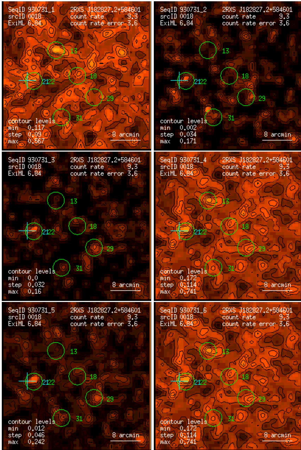
Figure 18: RASS 930731: detection 0018: band rate images, Gaussian filter: (1) PSPC channels 11 – 41, (2) 52 – 90, (3) 91 – 201, (4) 11 – 235, (5) 52 – 201, (6) 11 – 201. Broad band rates in counts/ks. Band rate contour levels in counts/ks/arcmin 2 .
