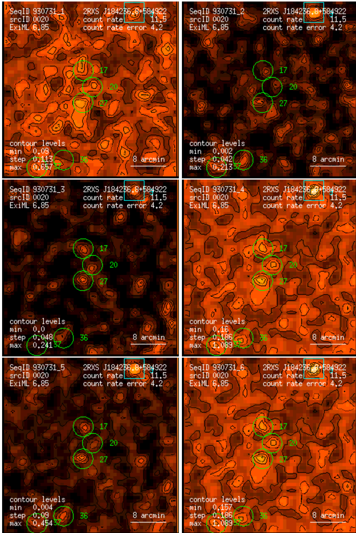
Figure 20: RASS 930731: detection 0020: band rate images, Gaussian filter: (1) PSPC channels 11 – 41, (2) 52 – 90, (3) 91 – 201, (4) 11 – 235, (5) 52 – 201, (6) 11 – 201. Broad band rates in counts/ks. Band rate contour levels in counts/ks/arcmin 2 .
