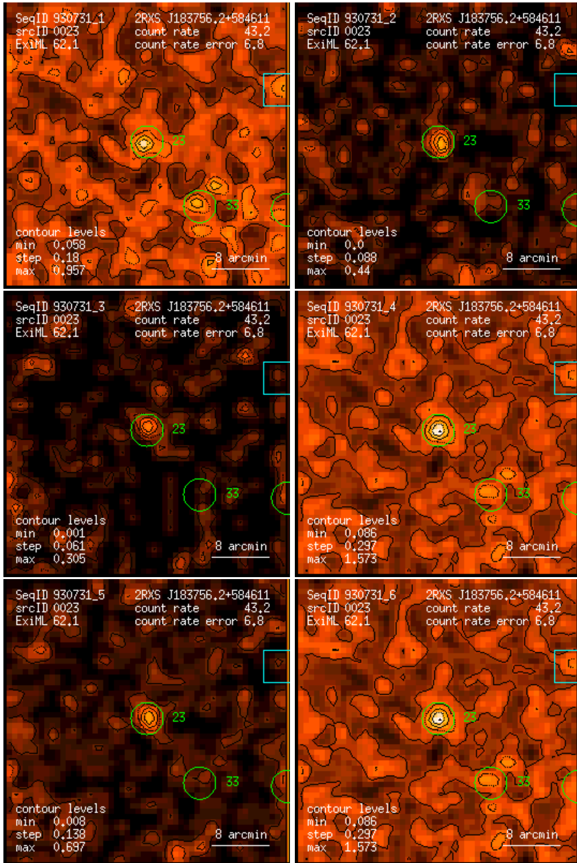
Figure 23: RASS 930731: detection 0023: band rate images, Gaussian filter: (1) PSPC channels 11 – 41, (2) 52 – 90, (3) 91 – 201, (4) 11 – 235, (5) 52 – 201, (6) 11 – 201. Broad band rates in counts/ks. Band rate contour levels in counts/ks/arcmin 2 .
