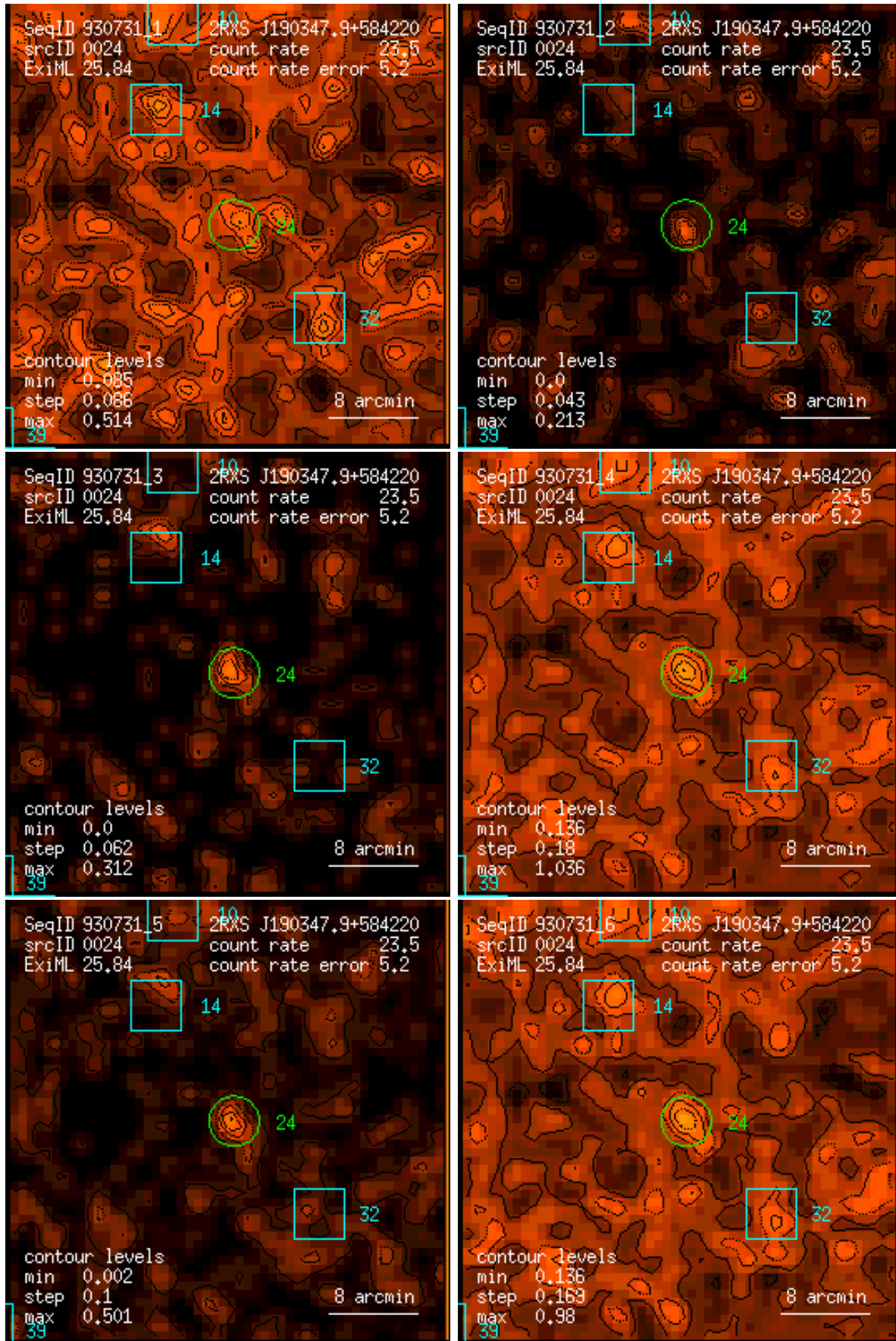
Figure 24: RASS 930731: detection 0024: band rate images, Gaussian filter: (1) PSPC channels 11 – 41, (2) 52 – 90, (3) 91 – 201, (4) 11 – 235, (5) 52 – 201, (6) 11 – 201. Broad band rates in counts/ks. Band rate contour levels in counts/ks/arcmin 2 .
