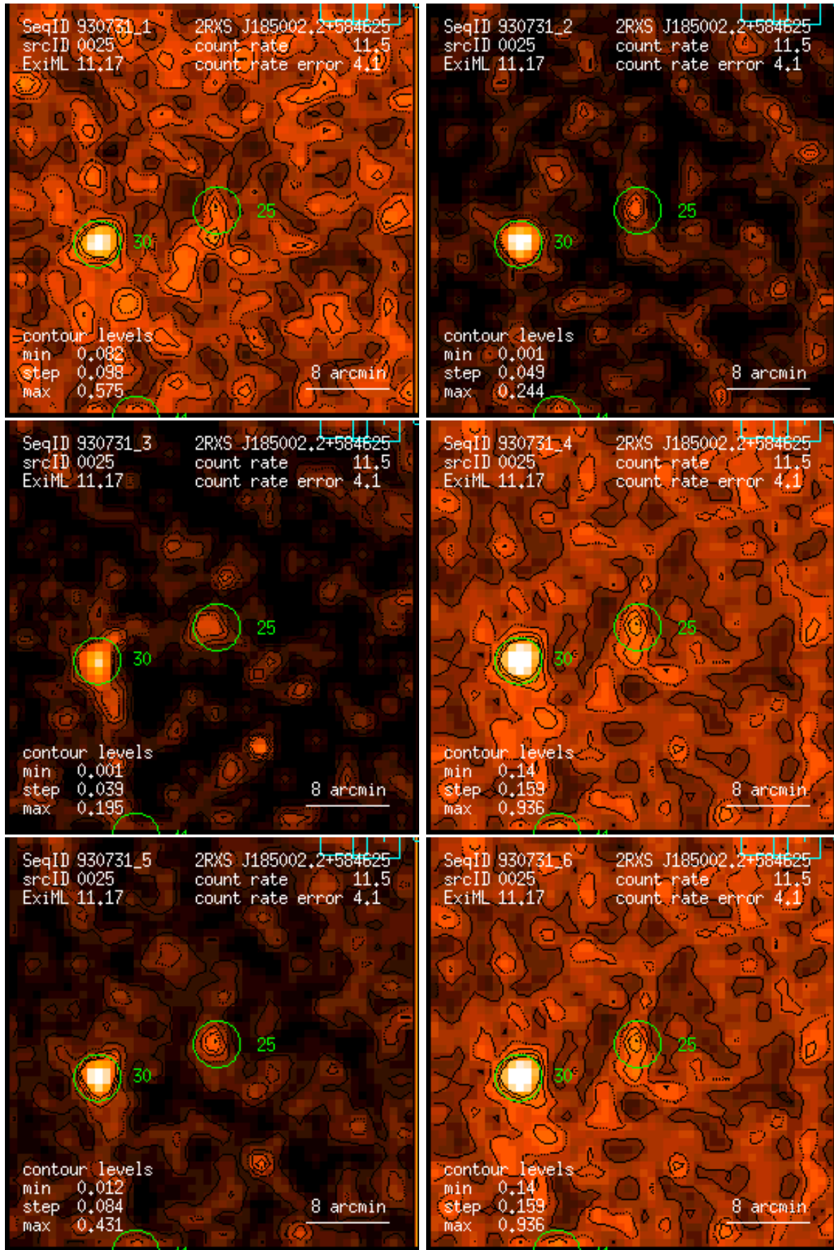
Figure 25: RASS 930731: detection 0025: band rate images, Gaussian filter: (1) PSPC channels 11 – 41, (2) 52 – 90, (3) 91 – 201, (4) 11 – 235, (5) 52 – 201, (6) 11 – 201. Broad band rates in counts/ks. Band rate contour levels in counts/ks/arcmin 2 .
