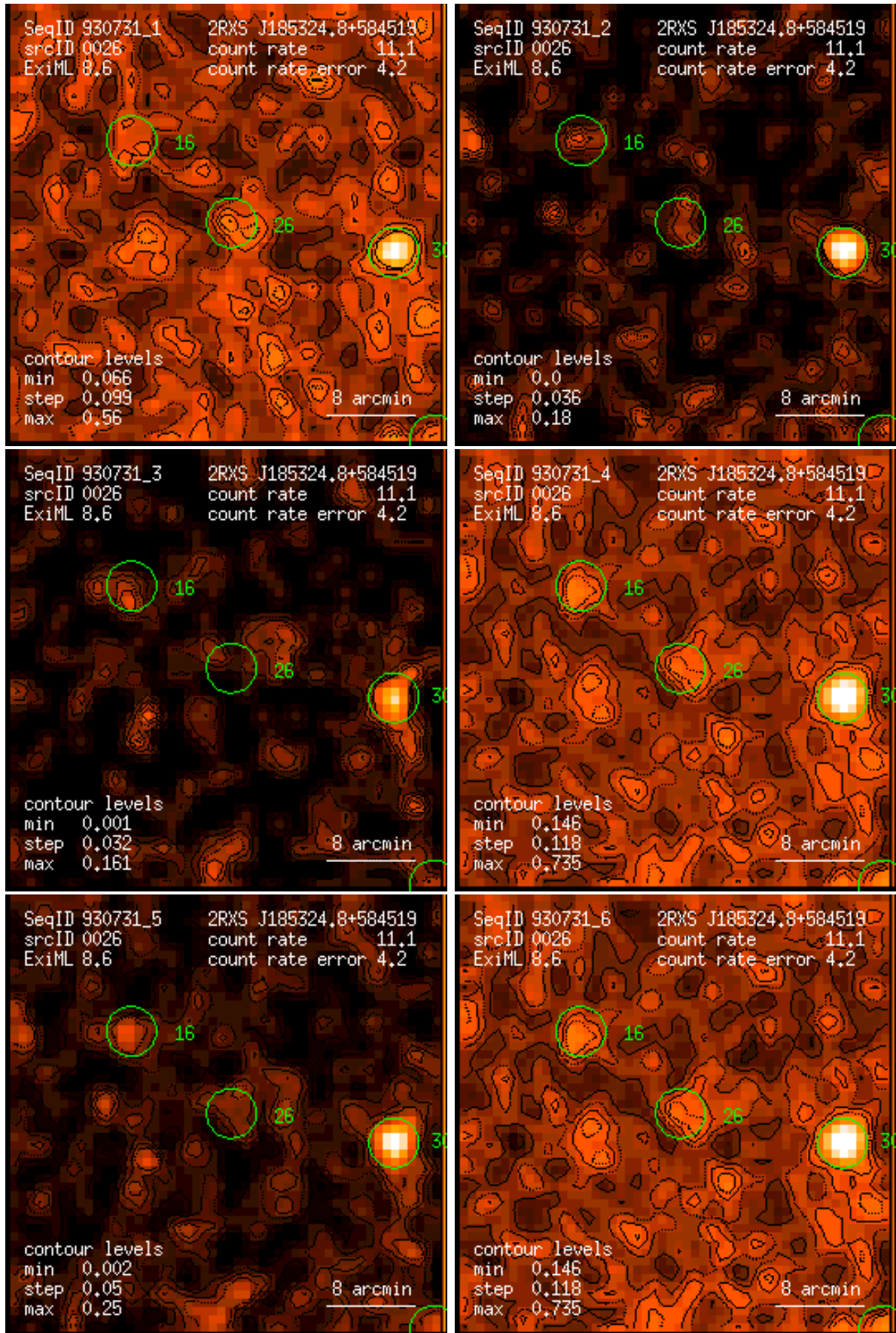
Figure 26: RASS 930731: detection 0026: band rate images, Gaussian filter: (1) PSPC channels 11 – 41, (2) 52 – 90, (3) 91 – 201, (4) 11 – 235, (5) 52 – 201, (6) 11 – 201. Broad band rates in counts/ks. Band rate contour levels in counts/ks/arcmin 2 .
