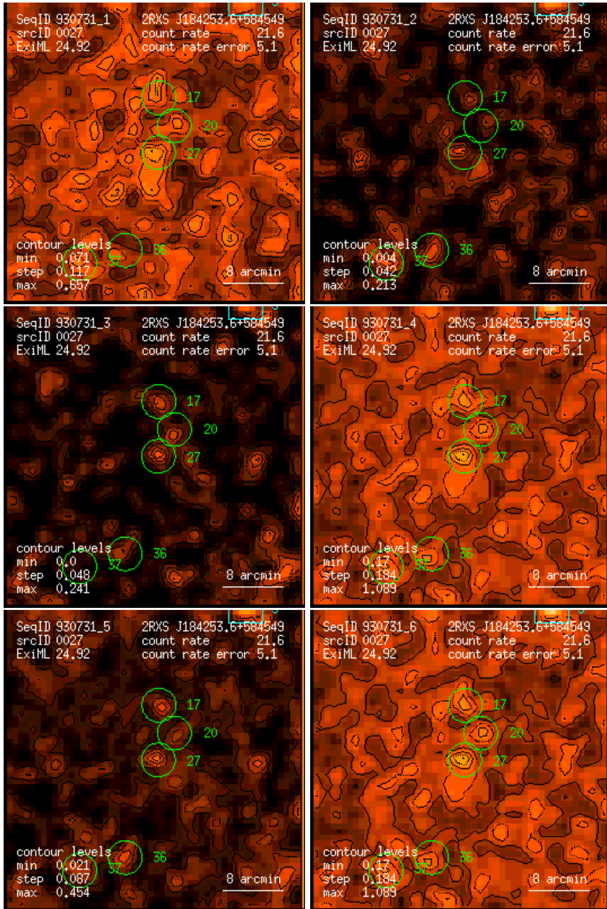
Figure 27: RASS 930731: detection 0027: band rate images, Gaussian filter: (1) PSPC channels 11 – 41, (2) 52 – 90, (3) 91 – 201, (4) 11 – 235, (5) 52 – 201, (6) 11 – 201. Broad band rates in counts/ks. Band rate contour levels in counts/ks/arcmin 2 .
