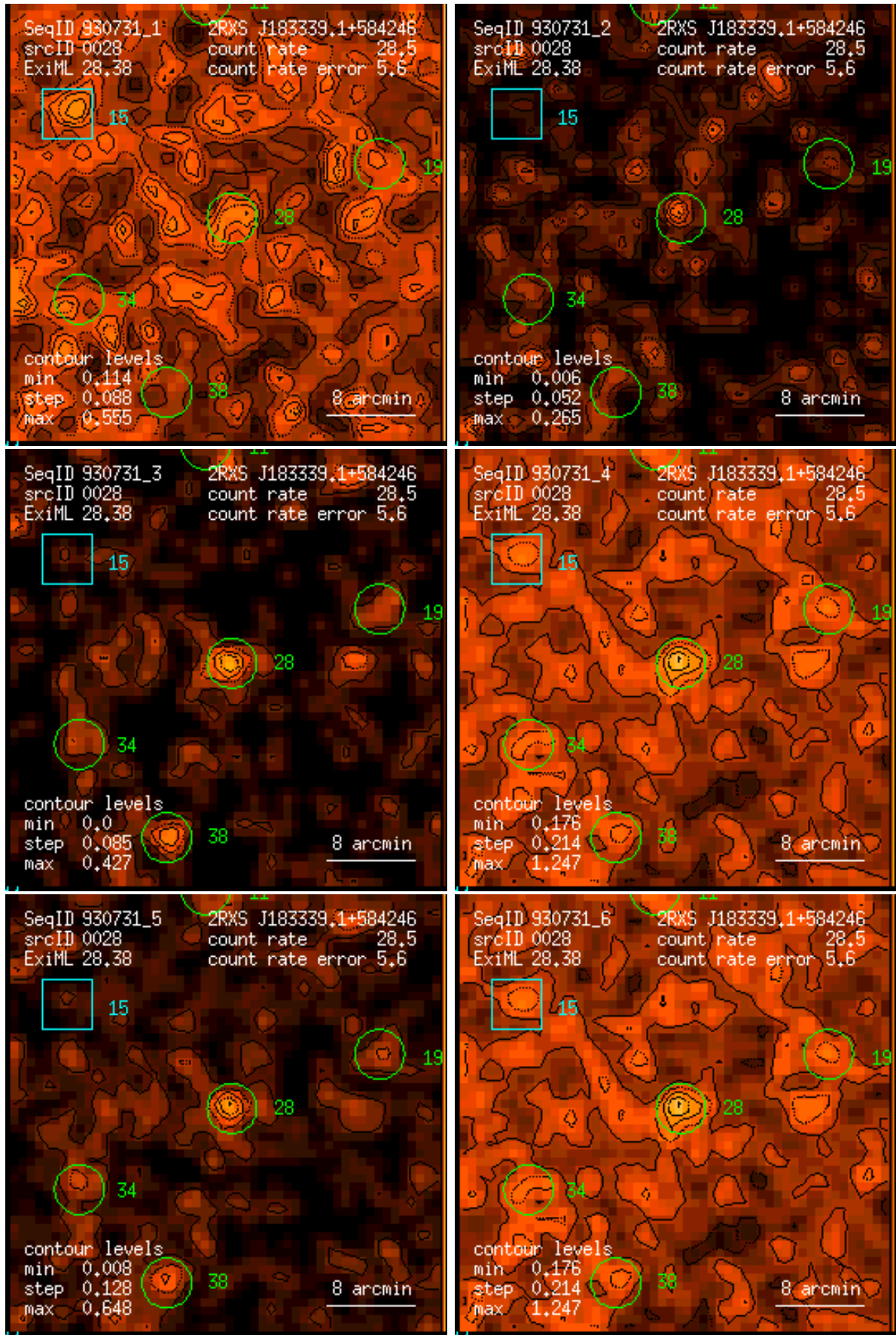
Figure 28: RASS 930731: detection 0028: band rate images, Gaussian filter: (1) PSPC channels 11 – 41, (2) 52 – 90, (3) 91 – 201, (4) 11 – 235, (5) 52 – 201, (6) 11 – 201. Broad band rates in counts/ks. Band rate contour levels in counts/ks/arcmin 2 .
