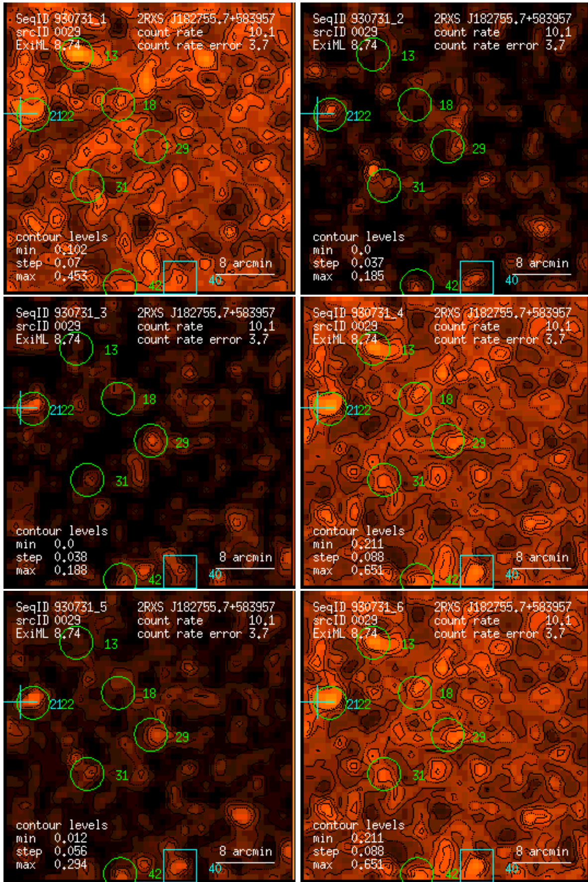
Figure 29: RASS 930731: detection 0029: band rate images, Gaussian filter: (1) PSPC channels 11 – 41, (2) 52 – 90, (3) 91 – 201, (4) 11 – 235, (5) 52 – 201, (6) 11 – 201. Broad band rates in counts/ks. Band rate contour levels in counts/ks/arcmin 2 .
