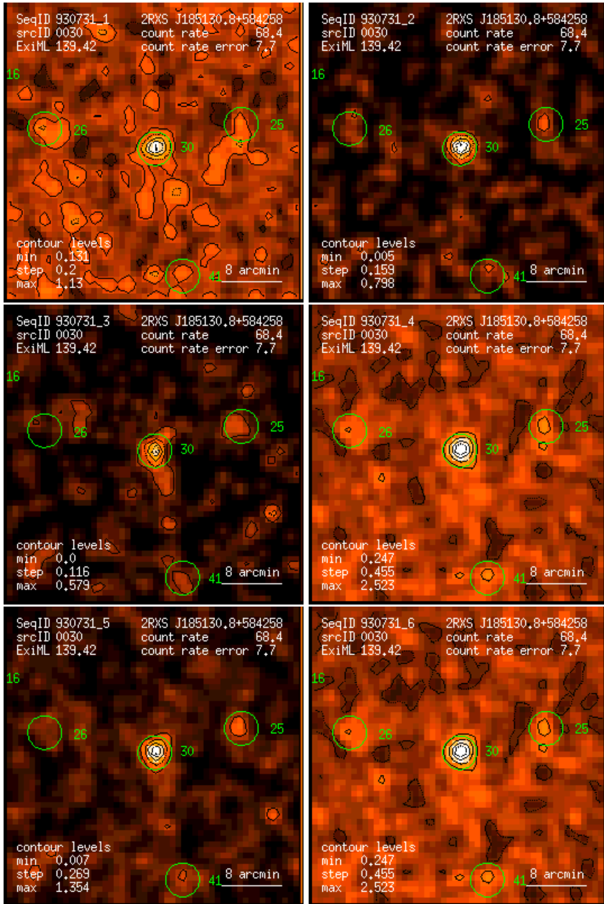
Figure 30: RASS 930731: detection 0030: band rate images, Gaussian filter: (1) PSPC channels 11 – 41, (2) 52 – 90, (3) 91 – 201, (4) 11 – 235, (5) 52 – 201, (6) 11 – 201. Broad band rates in counts/ks. Band rate contour levels in counts/ks/arcmin 2 .
