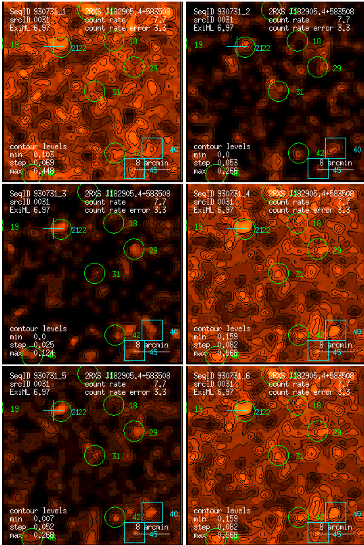
Figure 31: RASS 930731: detection 0031: band rate images, Gaussian filter: (1) PSPC channels 11 – 41, (2) 52 – 90, (3) 91 – 201, (4) 11 – 235, (5) 52 – 201, (6) 11 – 201. Broad band rates in counts/ks. Band rate contour levels in counts/ks/arcmin 2 .
