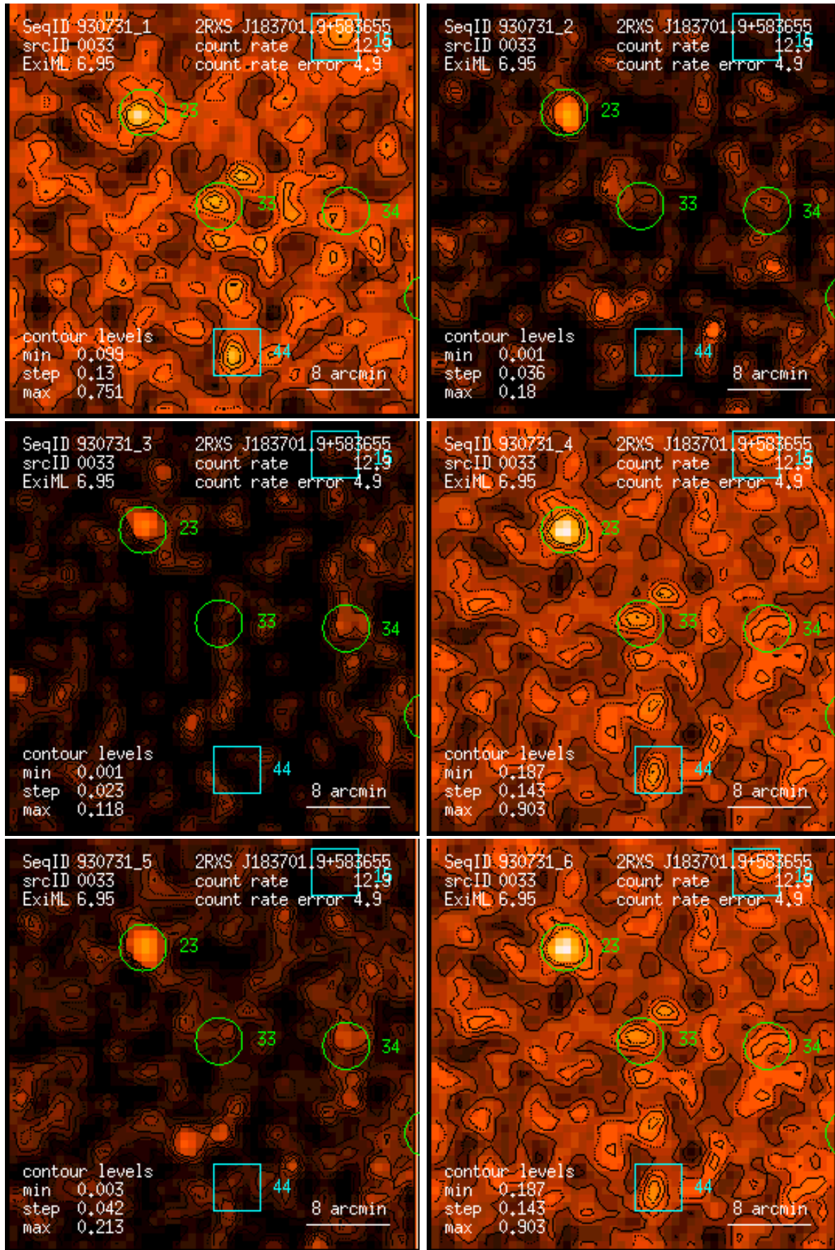
Figure 33: RASS 930731: detection 0033: band rate images, Gaussian filter: (1) PSPC channels 11 – 41, (2) 52 – 90, (3) 91 – 201, (4) 11 – 235, (5) 52 – 201, (6) 11 – 201. Broad band rates in counts/ks. Band rate contour levels in counts/ks/arcmin 2 .
