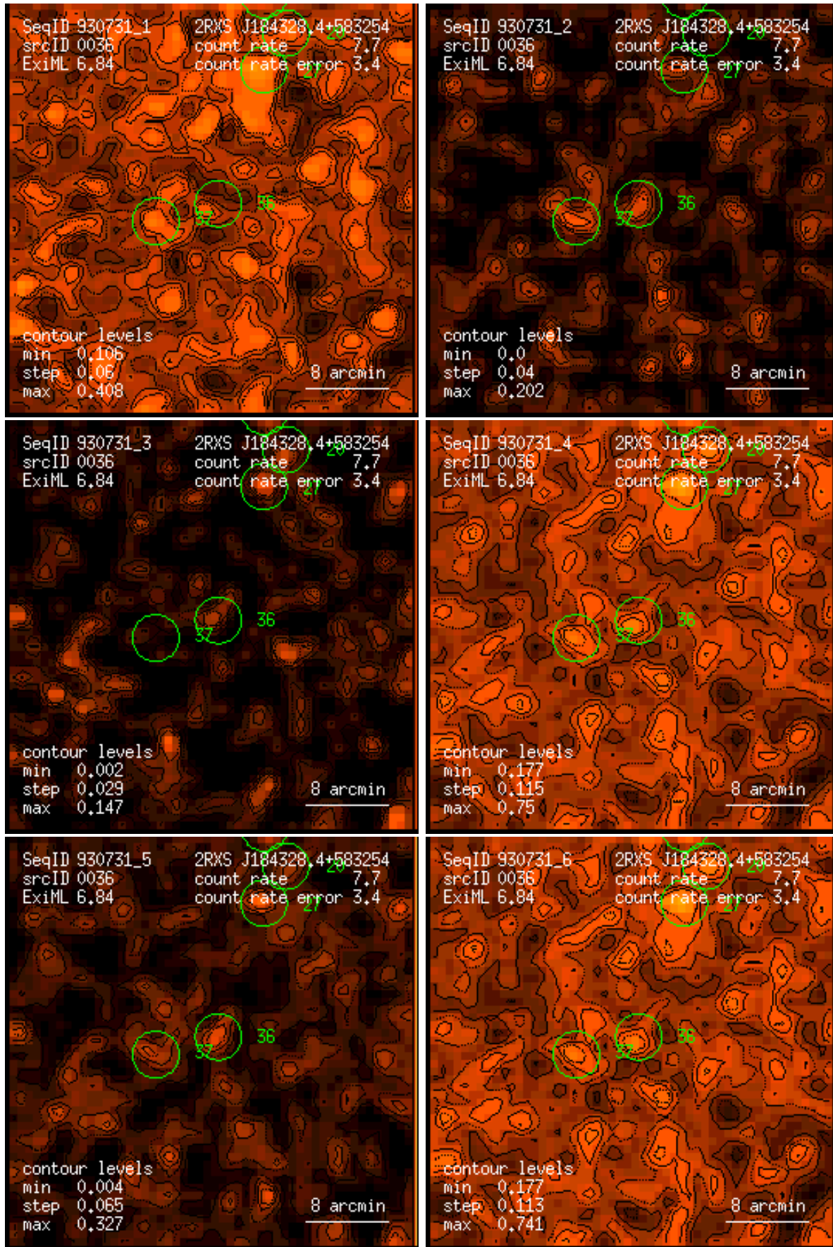
Figure 36: RASS 930731: detection 0036: band rate images, Gaussian filter: (1) PSPC channels 11 – 41, (2) 52 – 90, (3) 91 – 201, (4) 11 – 235, (5) 52 – 201, (6) 11 – 201. Broad band rates in counts/ks. Band rate contour levels in counts/ks/arcmin 2 .
