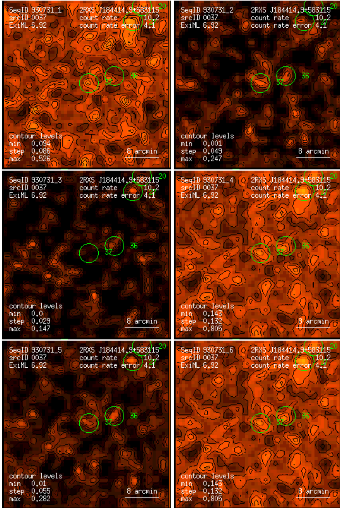
Figure 37: RASS 930731: detection 0037: band rate images, Gaussian filter: (1) PSPC channels 11 – 41, (2) 52 – 90, (3) 91 – 201, (4) 11 – 235, (5) 52 – 201, (6) 11 – 201. Broad band rates in counts/ks. Band rate contour levels in counts/ks/arcmin 2 .
