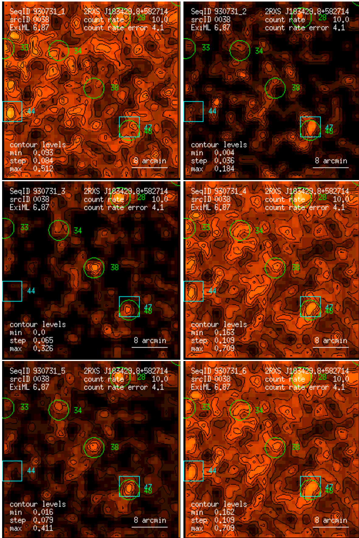
Figure 38: RASS 930731: detection 0038: band rate images, Gaussian filter: (1) PSPC channels 11 – 41, (2) 52 – 90, (3) 91 – 201, (4) 11 – 235, (5) 52 – 201, (6) 11 – 201. Broad band rates in counts/ks. Band rate contour levels in counts/ks/arcmin 2 .
