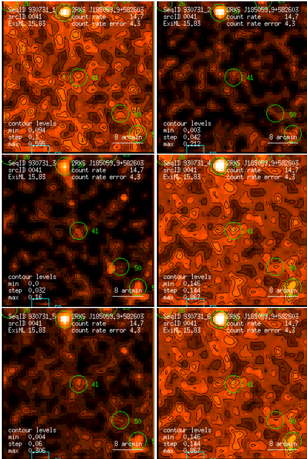
Figure 41: RASS 930731: detection 0041: band rate images, Gaussian filter: (1) PSPC channels 11 – 41, (2) 52 – 90, (3) 91 – 201, (4) 11 – 235, (5) 52 – 201, (6) 11 – 201. Broad band rates in counts/ks. Band rate contour levels in counts/ks/arcmin 2 .
