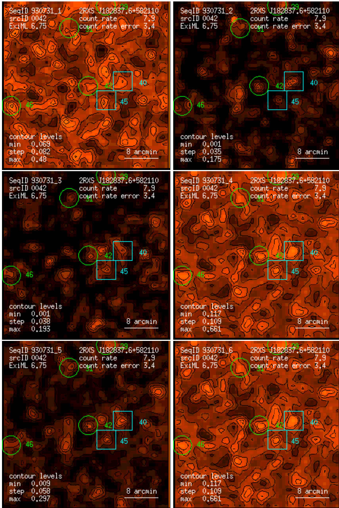
Figure 42: RASS 930731: detection 0042: band rate images, Gaussian filter: (1) PSPC channels 11 – 41, (2) 52 – 90, (3) 91 – 201, (4) 11 – 235, (5) 52 – 201, (6) 11 – 201. Broad band rates in counts/ks. Band rate contour levels in counts/ks/arcmin 2 .
