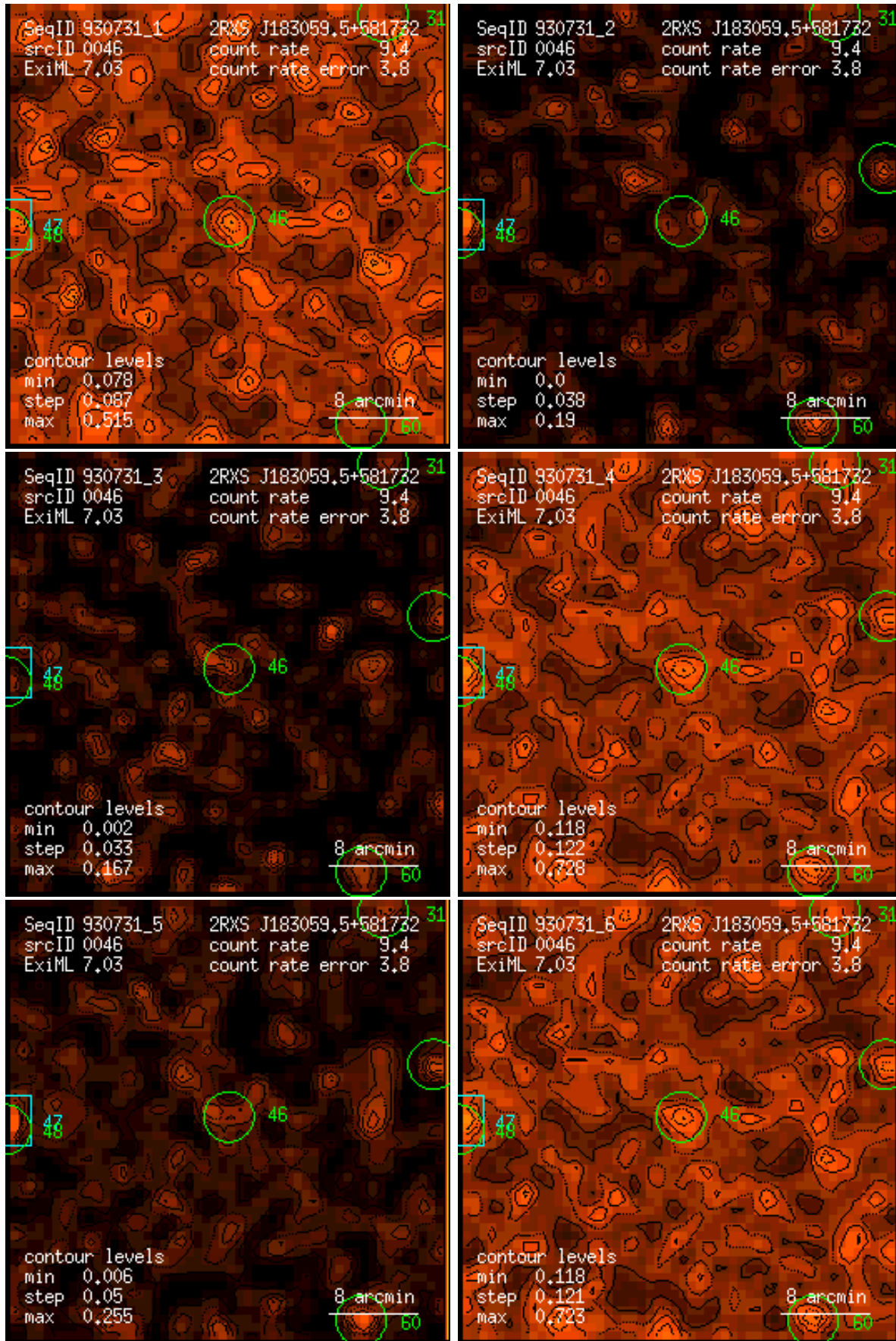
Figure 46: RASS 930731: detection 0046: band rate images, Gaussian filter: (1) PSPC channels 11 – 41, (2) 52 – 90, (3) 91 – 201, (4) 11 – 235, (5) 52 – 201, (6) 11 – 201. Broad band rates in counts/ks. Band rate contour levels in counts/ks/arcmin 2 .
