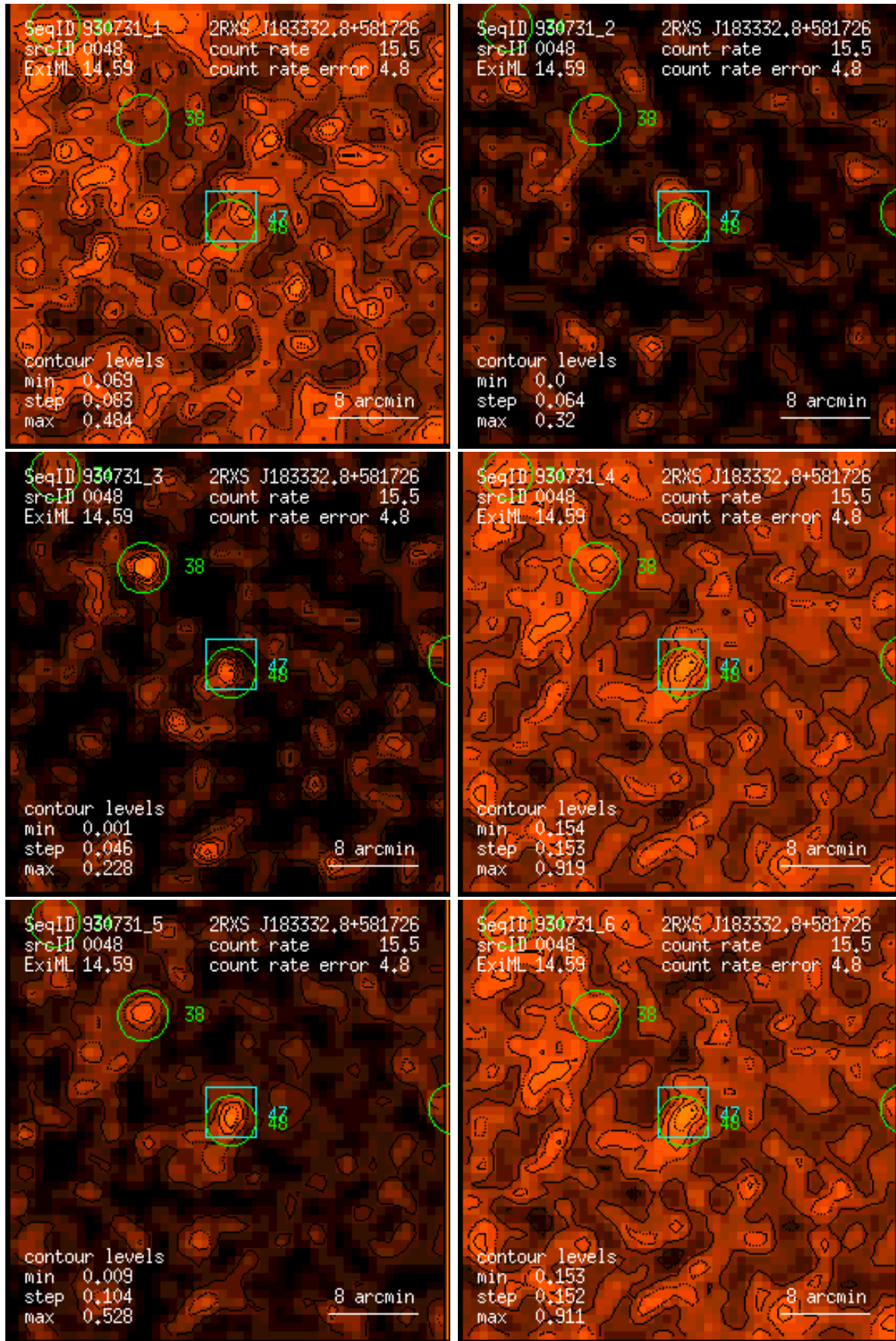
Figure 48: RASS 930731: detection 0048: band rate images, Gaussian filter: (1) PSPC channels 11 – 41, (2) 52 – 90, (3) 91 – 201, (4) 11 – 235, (5) 52 – 201, (6) 11 – 201. Broad band rates in counts/ks. Band rate contour levels in counts/ks/arcmin 2 .
