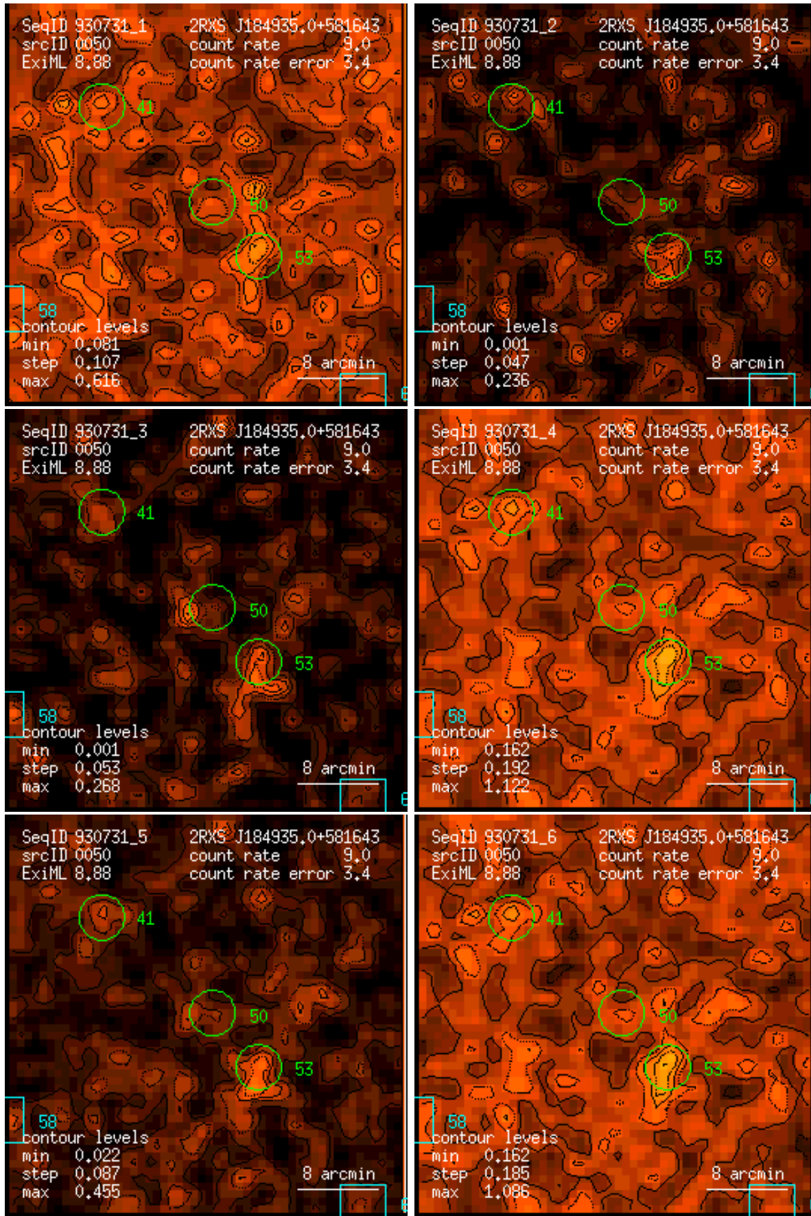
Figure 50: RASS 930731: detection 0050: band rate images, Gaussian filter: (1) PSPC channels 11 – 41, (2) 52 – 90, (3) 91 – 201, (4) 11 – 235, (5) 52 – 201, (6) 11 – 201. Broad band rates in counts/ks. Band rate contour levels in counts/ks/arcmin 2 .
