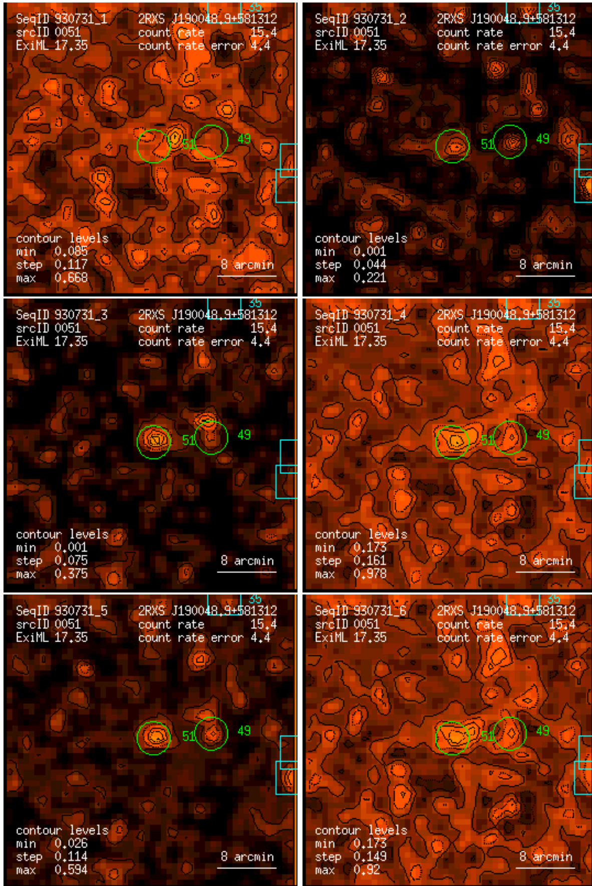
Figure 51: RASS 930731: detection 0051: band rate images, Gaussian filter: (1) PSPC channels 11 – 41, (2) 52 – 90, (3) 91 – 201, (4) 11 – 235, (5) 52 – 201, (6) 11 – 201. Broad band rates in counts/ks. Band rate contour levels in counts/ks/arcmin 2 .
