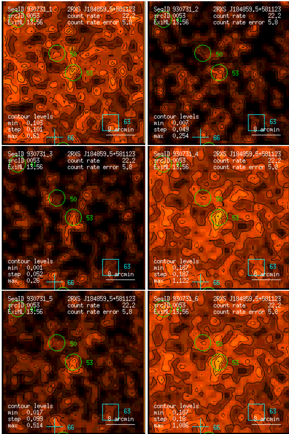
Figure 53: RASS 930731: detection 0053: band rate images, Gaussian filter: (1) PSPC channels 11 – 41, (2) 52 – 90, (3) 91 – 201, (4) 11 – 235, (5) 52 – 201, (6) 11 – 201. Broad band rates in counts/ks. Band rate contour levels in counts/ks/arcmin 2 .
