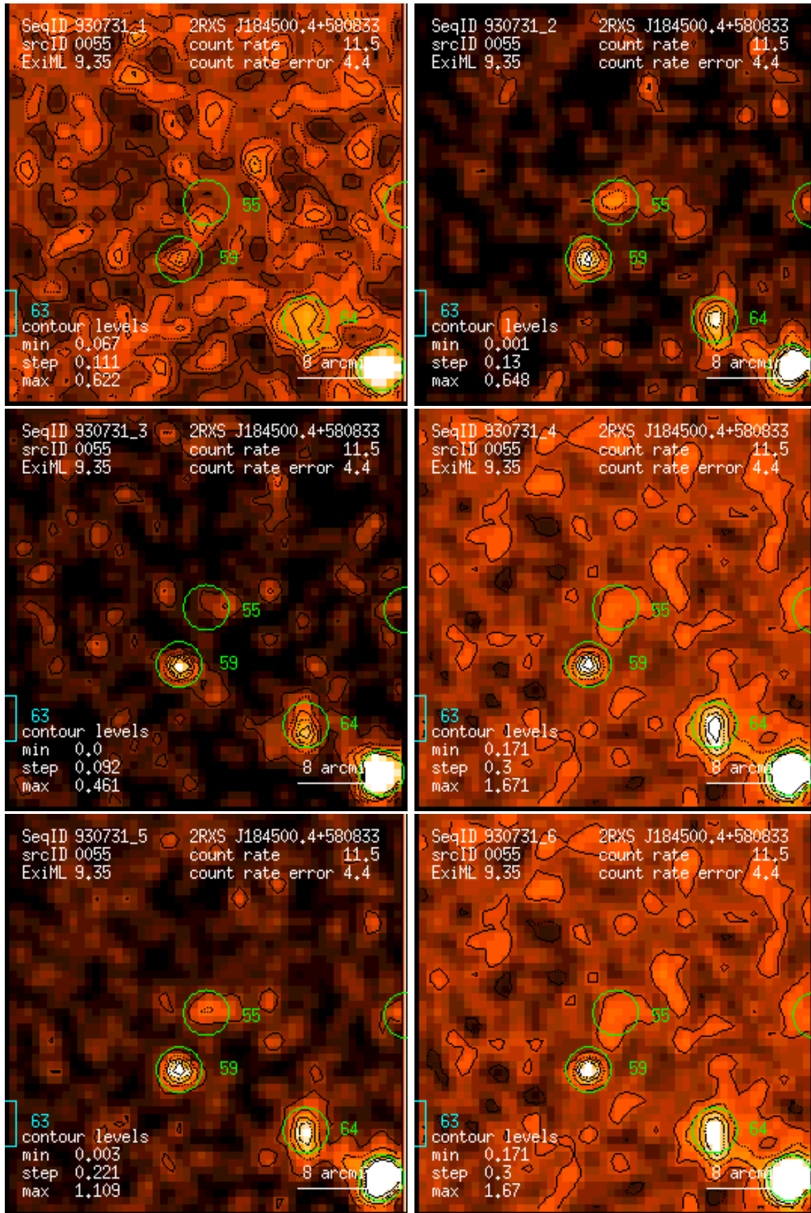
Figure 55: RASS 930731: detection 0055: band rate images, Gaussian filter: (1) PSPC channels 11 – 41, (2) 52 – 90, (3) 91 – 201, (4) 11 – 235, (5) 52 – 201, (6) 11 – 201. Broad band rates in counts/ks. Band rate contour levels in counts/ks/arcmin 2 .
