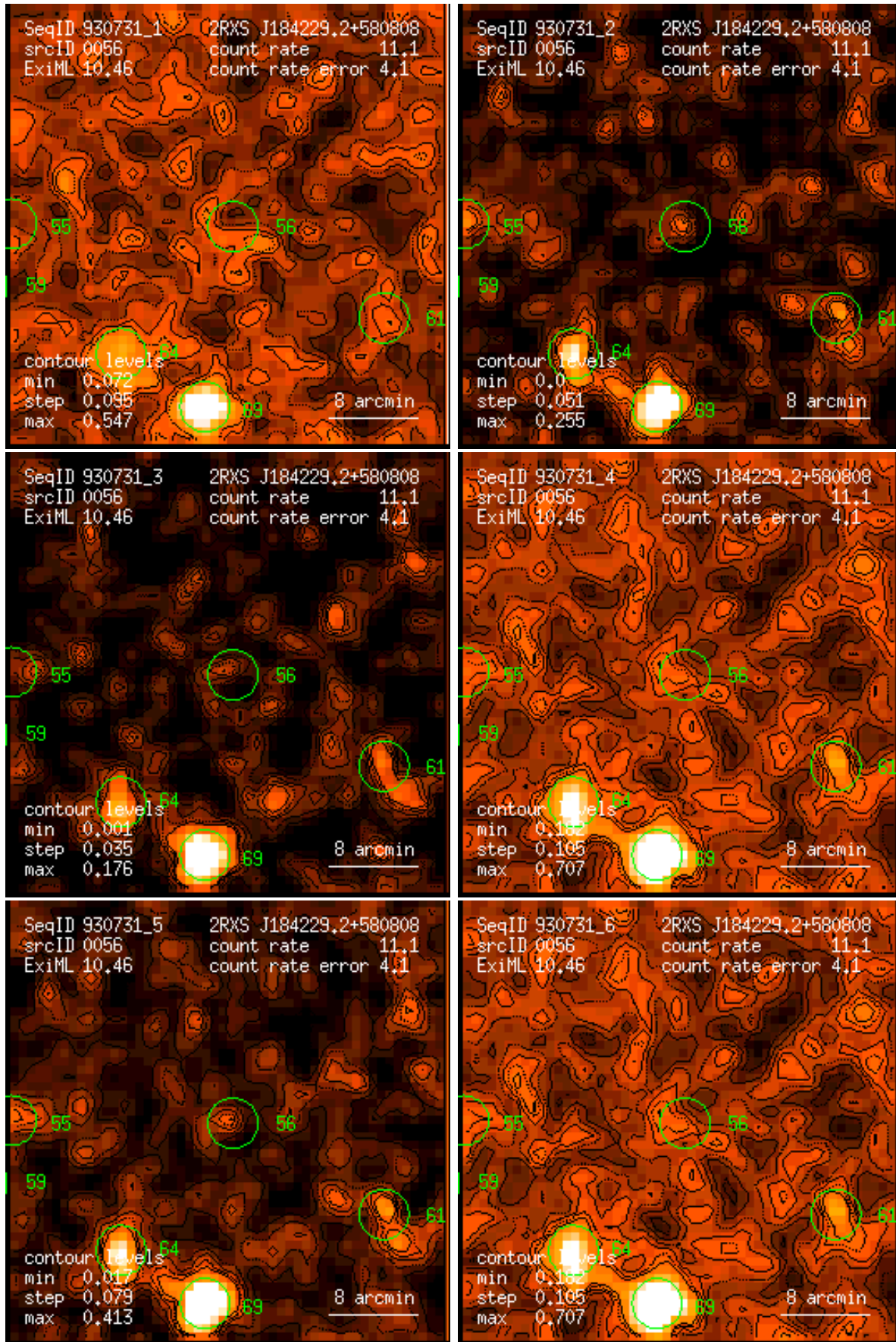
Figure 56: RASS 930731: detection 0056: band rate images, Gaussian filter: (1) PSPC channels 11 – 41, (2) 52 – 90, (3) 91 – 201, (4) 11 – 235, (5) 52 – 201, (6) 11 – 201. Broad band rates in counts/ks. Band rate contour levels in counts/ks/arcmin 2 .
