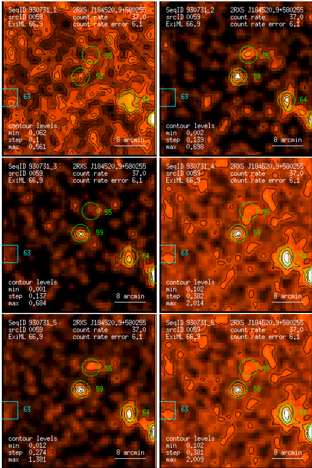
Figure 59: RASS 930731: detection 0059: band rate images, Gaussian filter: (1) PSPC channels 11 – 41, (2) 52 – 90, (3) 91 – 201, (4) 11 – 235, (5) 52 – 201, (6) 11 – 201. Broad band rates in counts/ks. Band rate contour levels in counts/ks/arcmin 2 .
