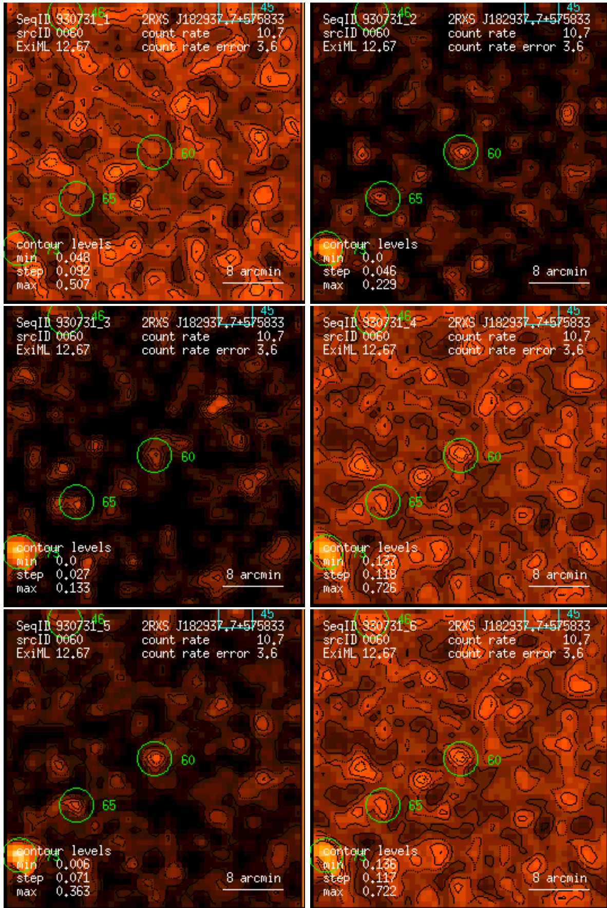
Figure 60: RASS 930731: detection 0060: band rate images, Gaussian filter: (1) PSPC channels 11 – 41, (2) 52 – 90, (3) 91 – 201, (4) 11 – 235, (5) 52 – 201, (6) 11 – 201. Broad band rates in counts/ks. Band rate contour levels in counts/ks/arcmin 2 .
