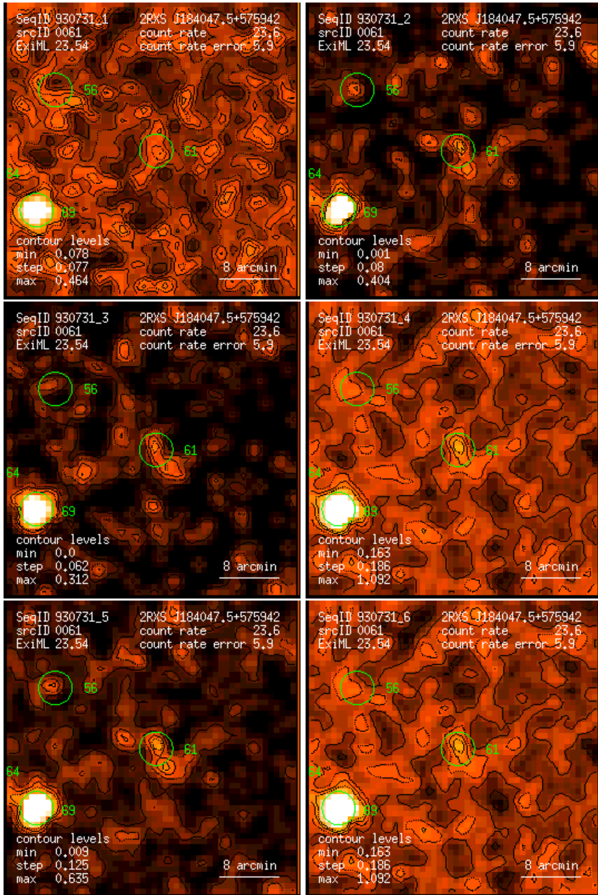
Figure 61: RASS 930731: detection 0061: band rate images, Gaussian filter: (1) PSPC channels 11 – 41, (2) 52 – 90, (3) 91 – 201, (4) 11 – 235, (5) 52 – 201, (6) 11 – 201. Broad band rates in counts/ks. Band rate contour levels in counts/ks/arcmin 2 .
