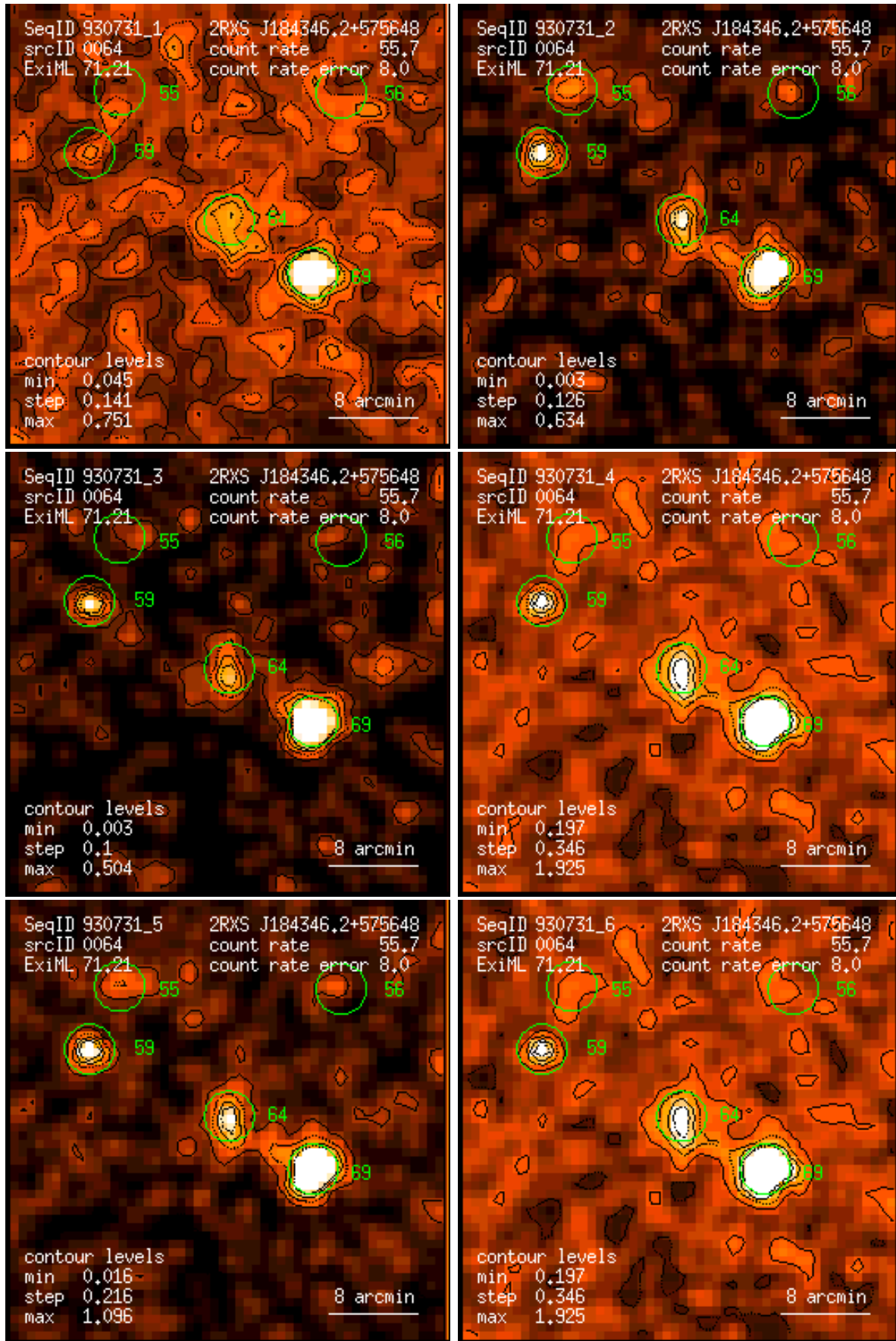
Figure 64: RASS 930731: detection 0064: band rate images, Gaussian filter: (1) PSPC channels 11 – 41, (2) 52 – 90, (3) 91 – 201, (4) 11 – 235, (5) 52 – 201, (6) 11 – 201. Broad band rates in counts/ks. Band rate contour levels in counts/ks/arcmin 2 .
