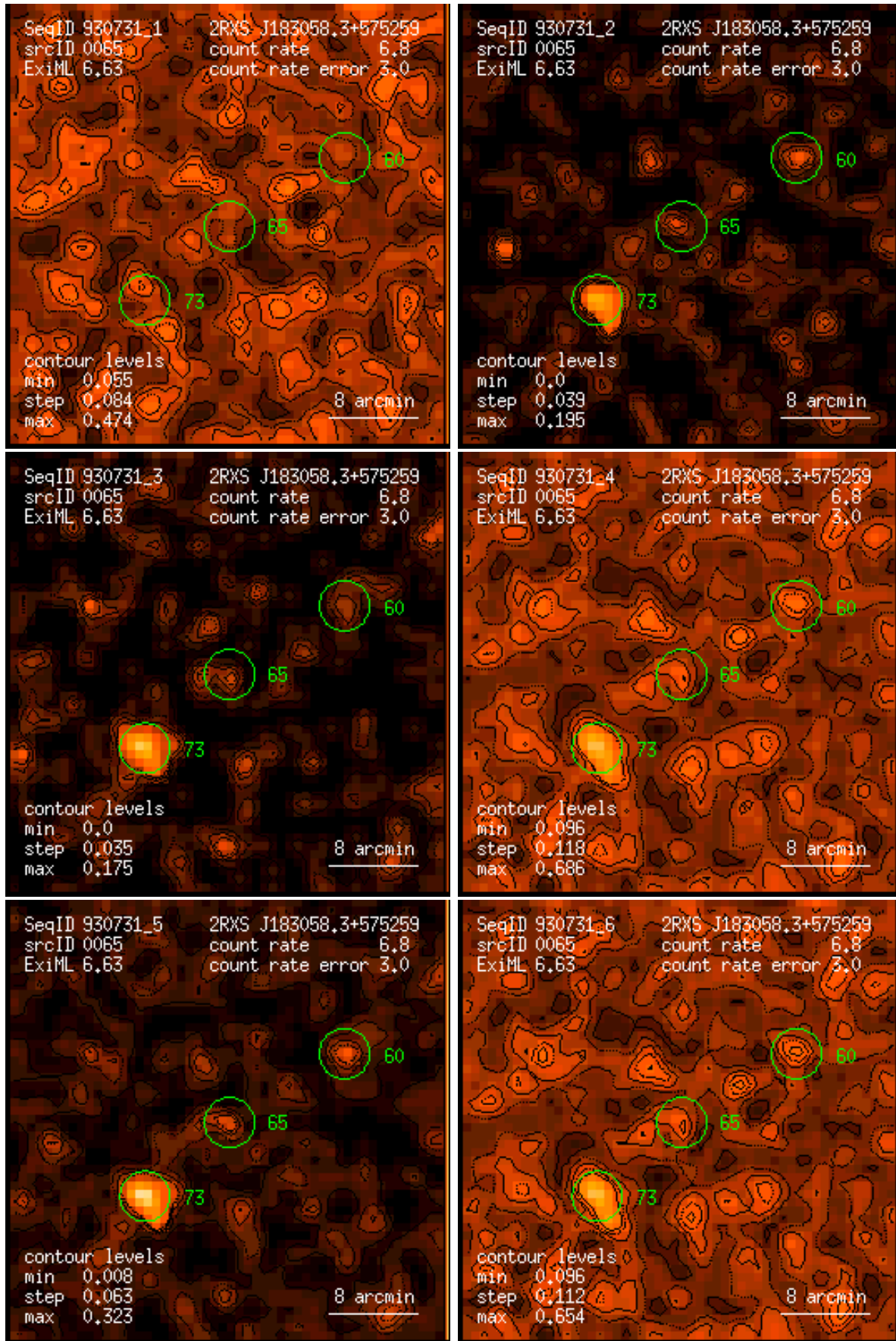
Figure 65: RASS 930731: detection 0065: band rate images, Gaussian filter: (1) PSPC channels 11 – 41, (2) 52 – 90, (3) 91 – 201, (4) 11 – 235, (5) 52 – 201, (6) 11 – 201. Broad band rates in counts/ks. Band rate contour levels in counts/ks/arcmin 2 .
